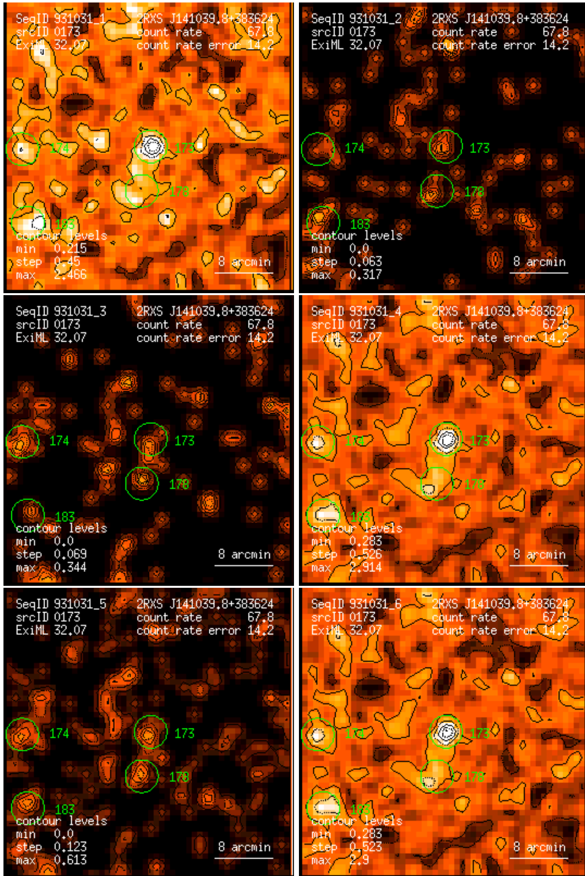
Figure 173: RASS 931031: detection 0173: band rate images, Gaussian filter: (1) PSPC channels 11 – 41, (2) 52 – 90, (3) 91 – 201, (4) 11 – 235, (5) 52 – 201, (6) 11 – 201. Broad band rates in counts/ks. Band rate contour levels in counts/ks/arcmin 2 .
