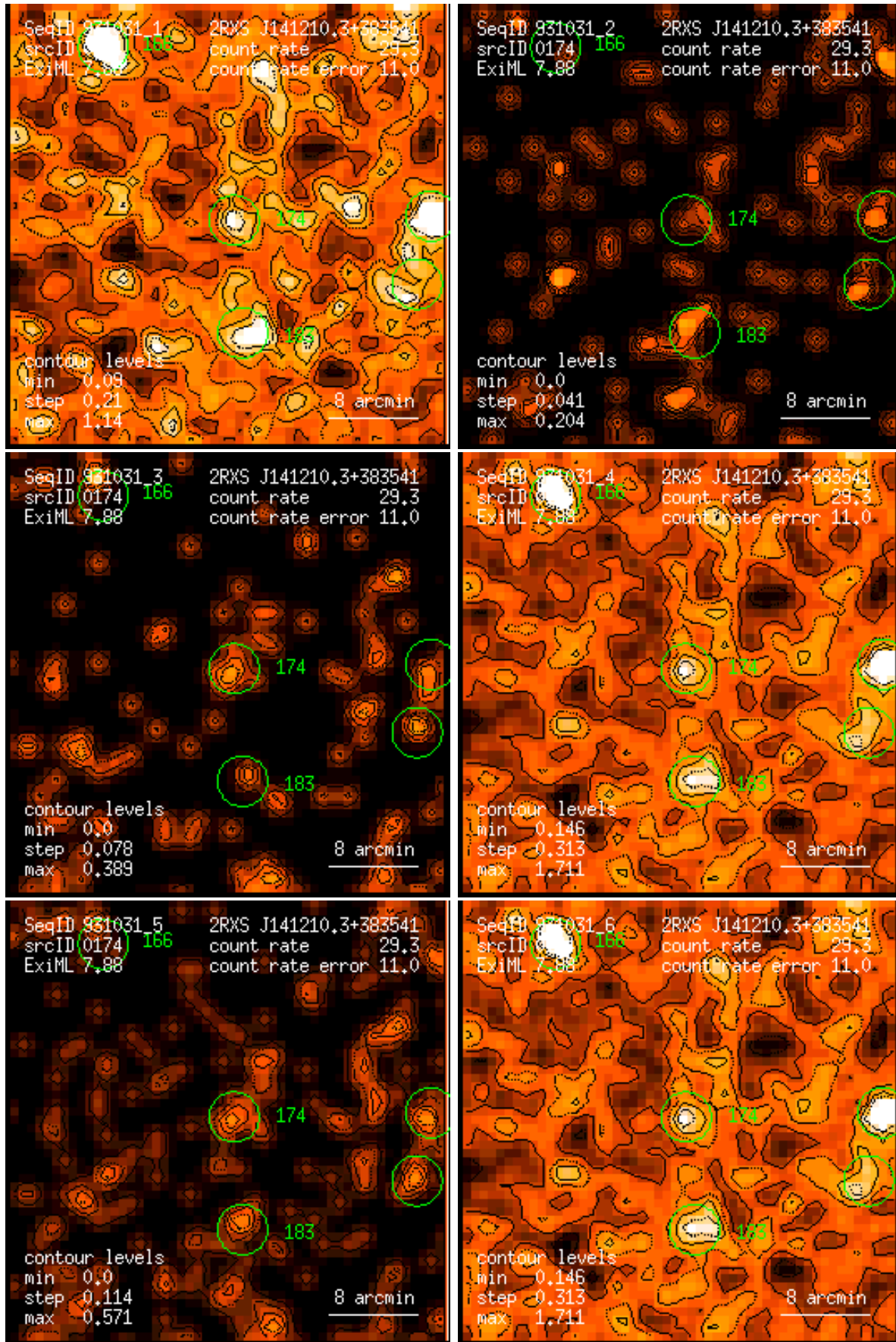
Figure 174: RASS 931031: detection 0174: band rate images, Gaussian filter: (1) PSPC channels 11 – 41, (2) 52 – 90, (3) 91 – 201, (4) 11 – 235, (5) 52 – 201, (6) 11 – 201. Broad band rates in counts/ks. Band rate contour levels in counts/ks/arcmin 2 .
