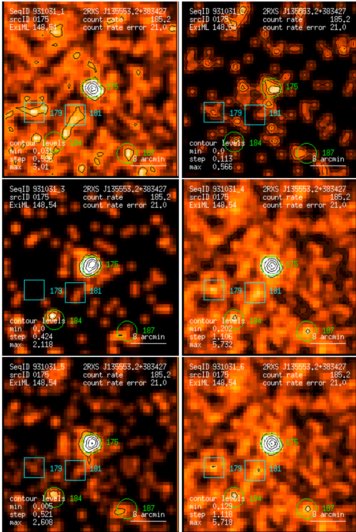
Figure 175: RASS 931031: detection 0175: band rate images, Gaussian filter: (1) PSPC channels 11 – 41, (2) 52 – 90, (3) 91 – 201, (4) 11 – 235, (5) 52 – 201, (6) 11 – 201. Broad band rates in counts/ks. Band rate contour levels in counts/ks/arcmin 2 .
