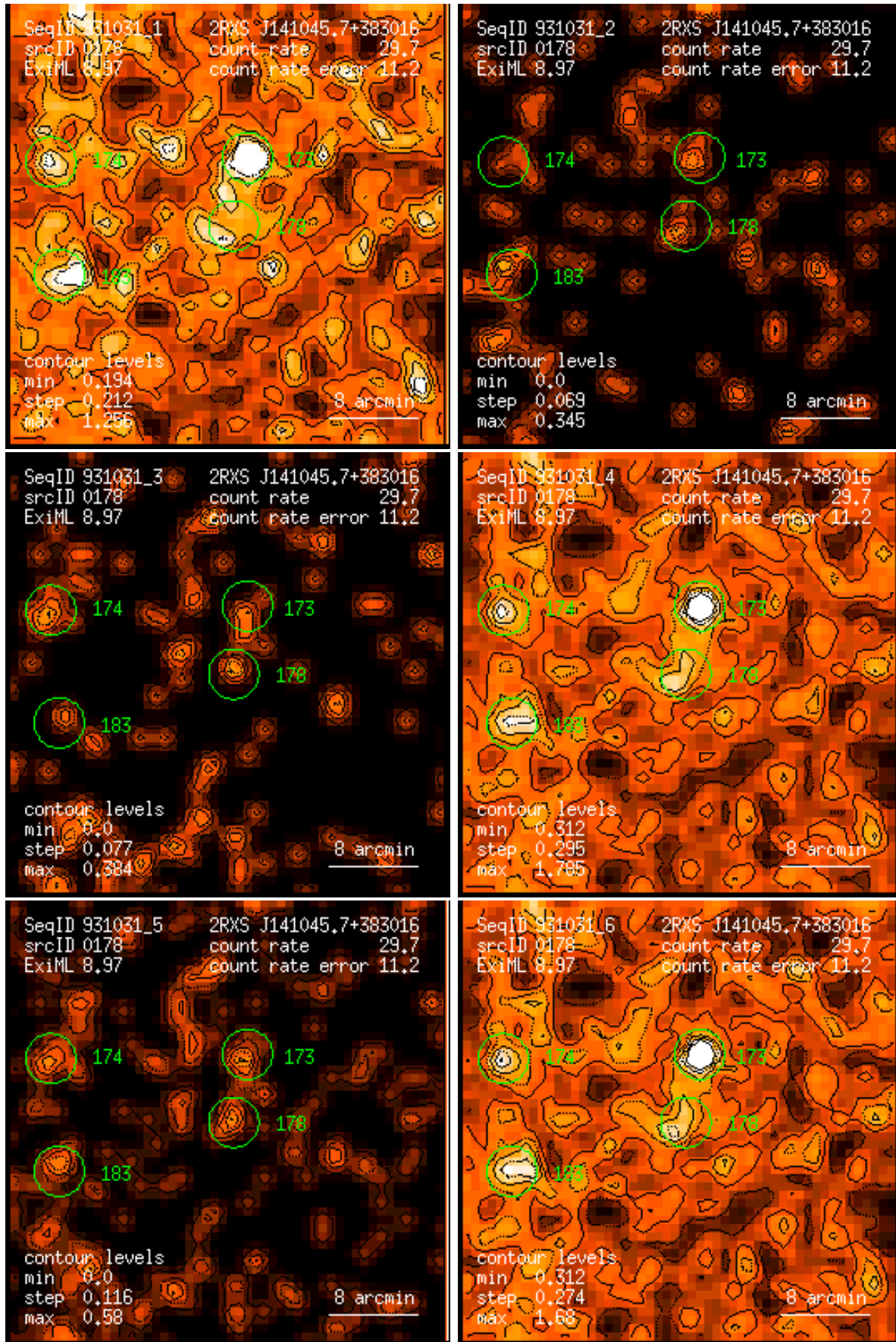
Figure 178: RASS 931031: detection 0178: band rate images, Gaussian filter: (1) PSPC channels 11 – 41, (2) 52 – 90, (3) 91 – 201, (4) 11 – 235, (5) 52 – 201, (6) 11 – 201. Broad band rates in counts/ks. Band rate contour levels in counts/ks/arcmin 2 .
