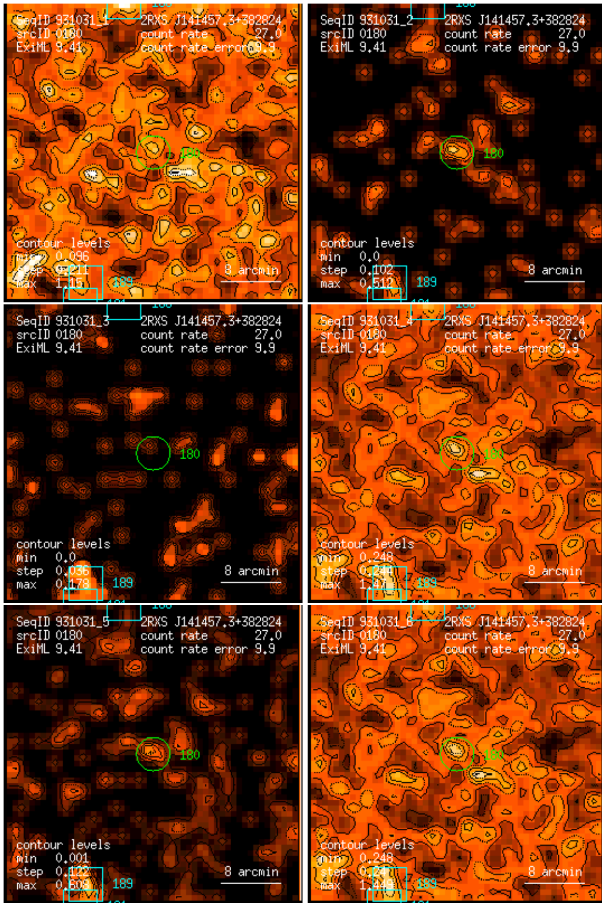
Figure 180: RASS 931031: detection 0180: band rate images, Gaussian filter: (1) PSPC channels 11 – 41, (2) 52 – 90, (3) 91 – 201, (4) 11 – 235, (5) 52 – 201, (6) 11 – 201. Broad band rates in counts/ks. Band rate contour levels in counts/ks/arcmin 2 .
