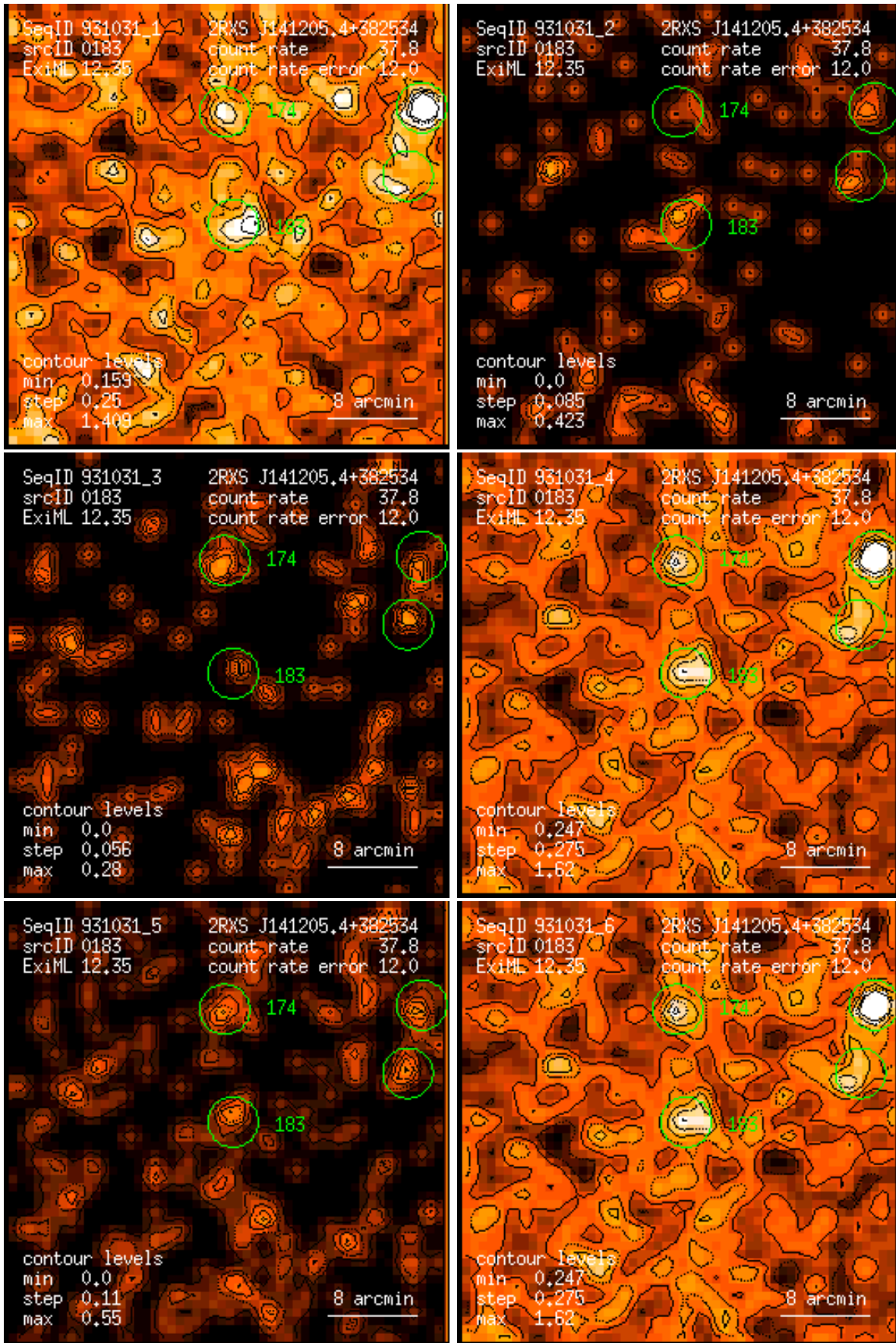
Figure 183: RASS 931031: detection 0183: band rate images, Gaussian filter: (1) PSPC channels 11 – 41, (2) 52 – 90, (3) 91 – 201, (4) 11 – 235, (5) 52 – 201, (6) 11 – 201. Broad band rates in counts/ks. Band rate contour levels in counts/ks/arcmin 2 .
