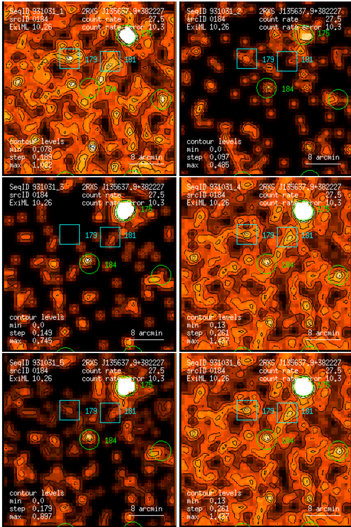
Figure 184: RASS 931031: detection 0184: band rate images, Gaussian filter: (1) PSPC channels 11 – 41, (2) 52 – 90, (3) 91 – 201, (4) 11 – 235, (5) 52 – 201, (6) 11 – 201. Broad band rates in counts/ks. Band rate contour levels in counts/ks/arcmin 2 .
