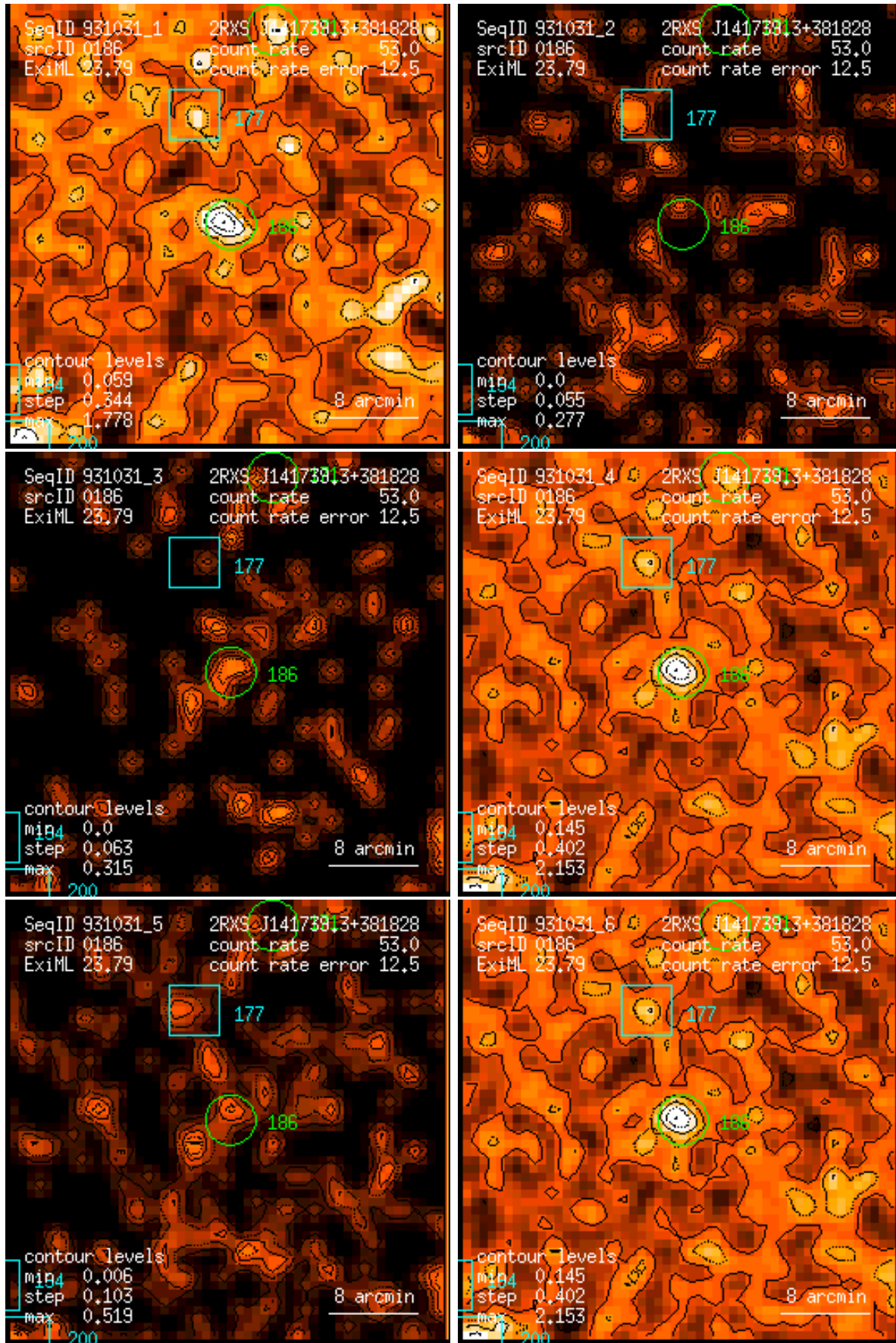
Figure 186: RASS 931031: detection 0186: band rate images, Gaussian filter: (1) PSPC channels 11 – 41, (2) 52 – 90, (3) 91 – 201, (4) 11 – 235, (5) 52 – 201, (6) 11 – 201. Broad band rates in counts/ks. Band rate contour levels in counts/ks/arcmin 2 .
