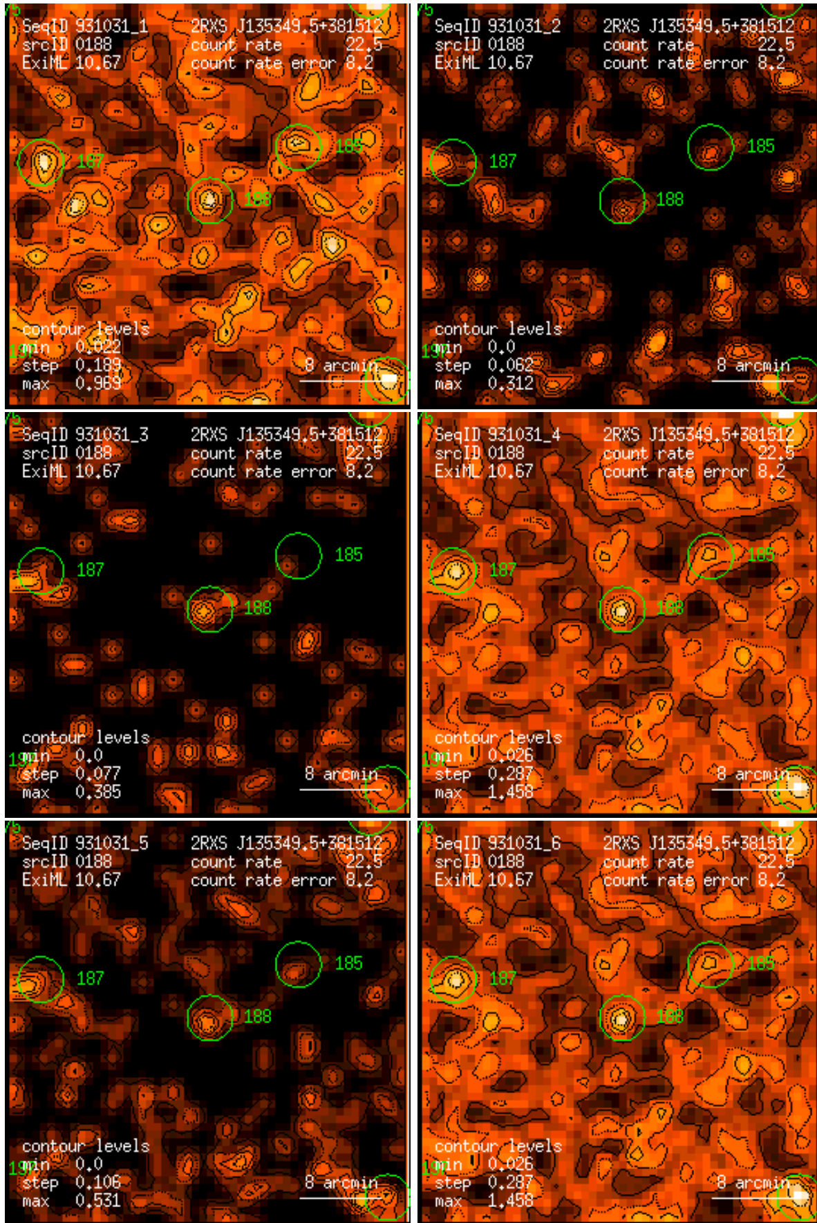
Figure 188: RASS 931031: detection 0188: band rate images, Gaussian filter: (1) PSPC channels 11 – 41, (2) 52 – 90, (3) 91 – 201, (4) 11 – 235, (5) 52 – 201, (6) 11 – 201. Broad band rates in counts/ks. Band rate contour levels in counts/ks/arcmin 2 .
