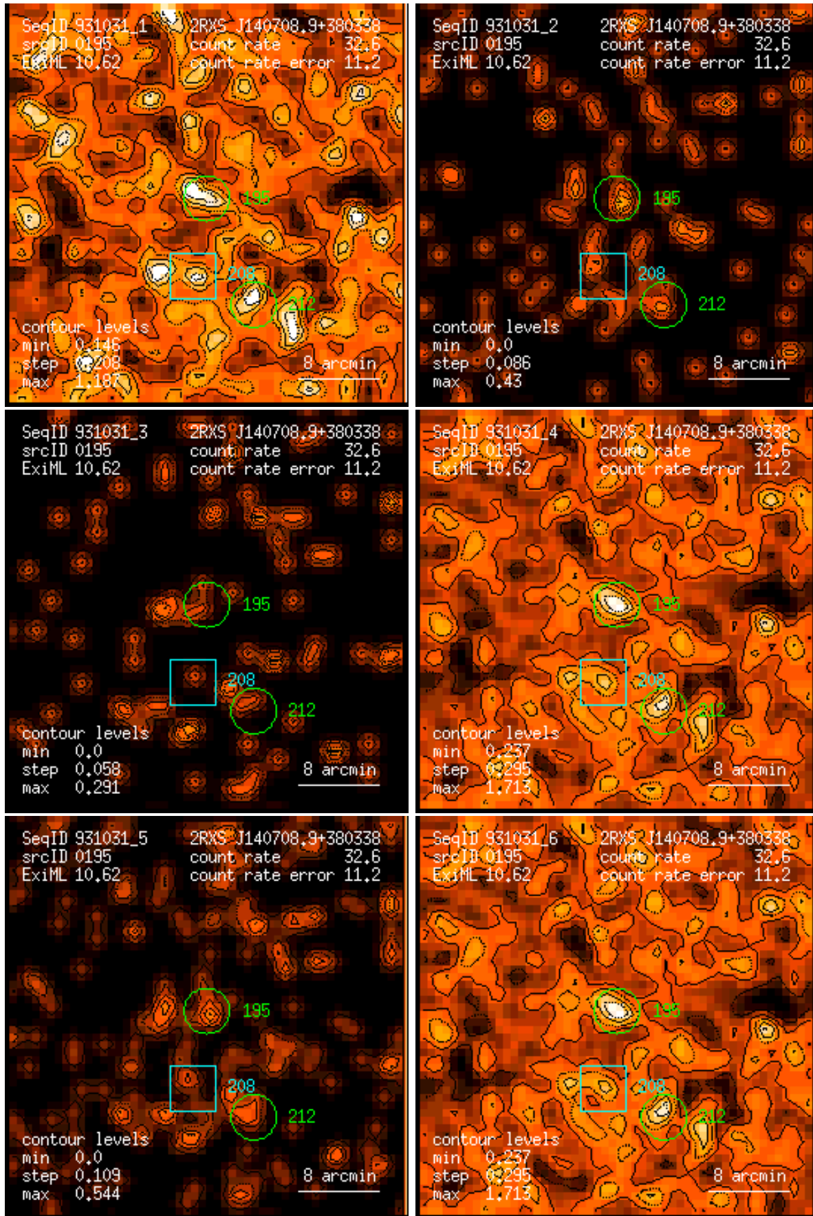
Figure 195: RASS 931031: detection 0195: band rate images, Gaussian filter: (1) PSPC channels 11 – 41, (2) 52 – 90, (3) 91 – 201, (4) 11 – 235, (5) 52 – 201, (6) 11 – 201. Broad band rates in counts/ks. Band rate contour levels in counts/ks/arcmin 2 .
