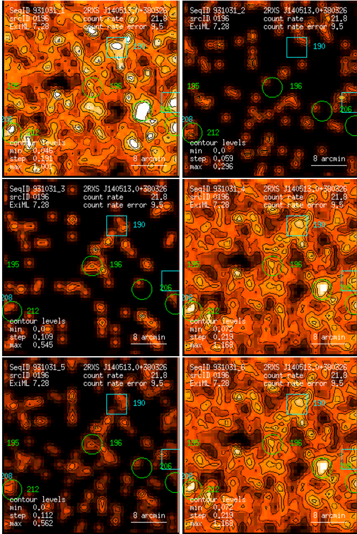
Figure 196: RASS 931031: detection 0196: band rate images, Gaussian filter: (1) PSPC channels 11 – 41, (2) 52 – 90, (3) 91 – 201, (4) 11 – 235, (5) 52 – 201, (6) 11 – 201. Broad band rates in counts/ks. Band rate contour levels in counts/ks/arcmin 2 .
