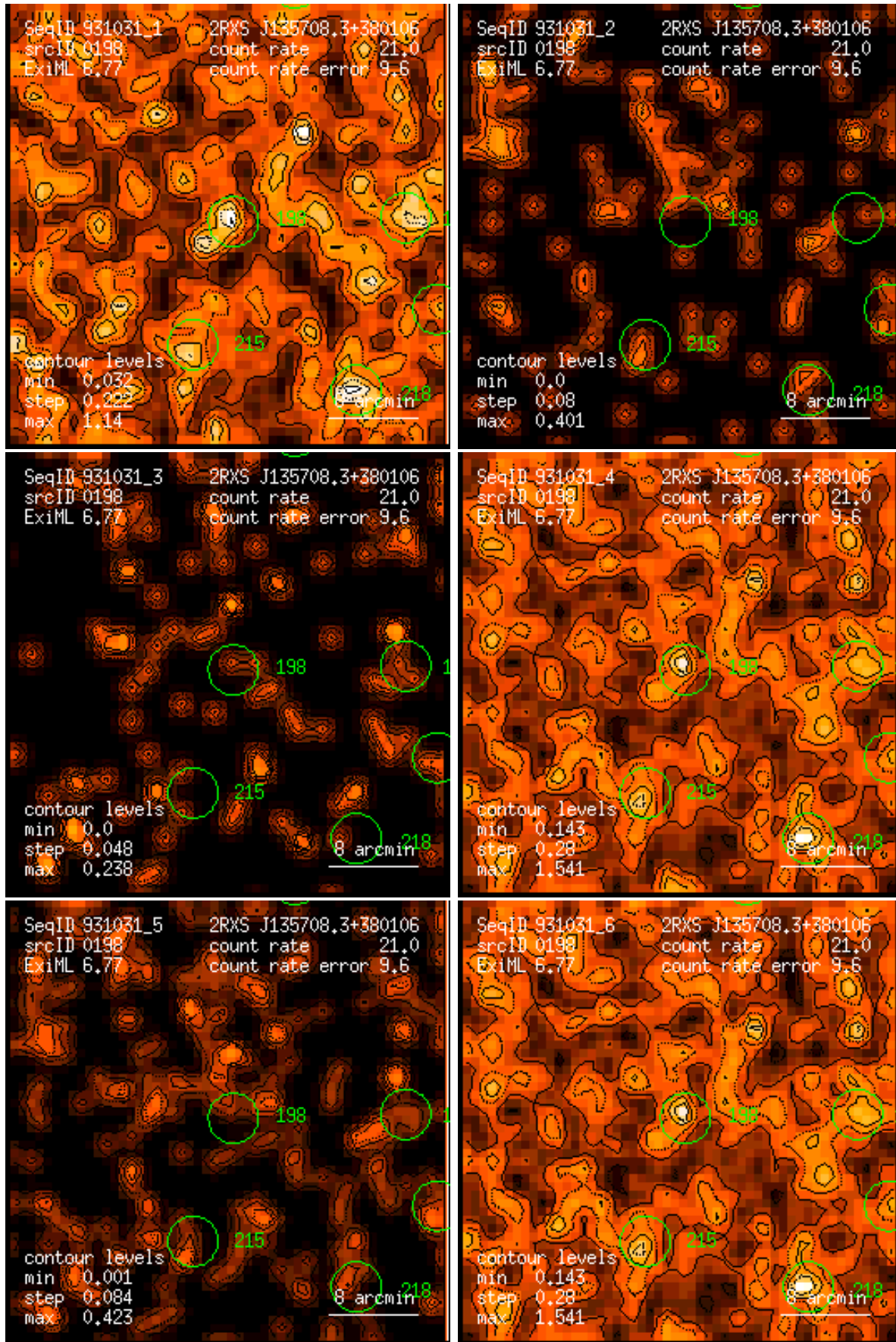
Figure 198: RASS 931031: detection 0198: band rate images, Gaussian filter: (1) PSPC channels 11 – 41, (2) 52 – 90, (3) 91 – 201, (4) 11 – 235, (5) 52 – 201, (6) 11 – 201. Broad band rates in counts/ks. Band rate contour levels in counts/ks/arcmin 2 .
