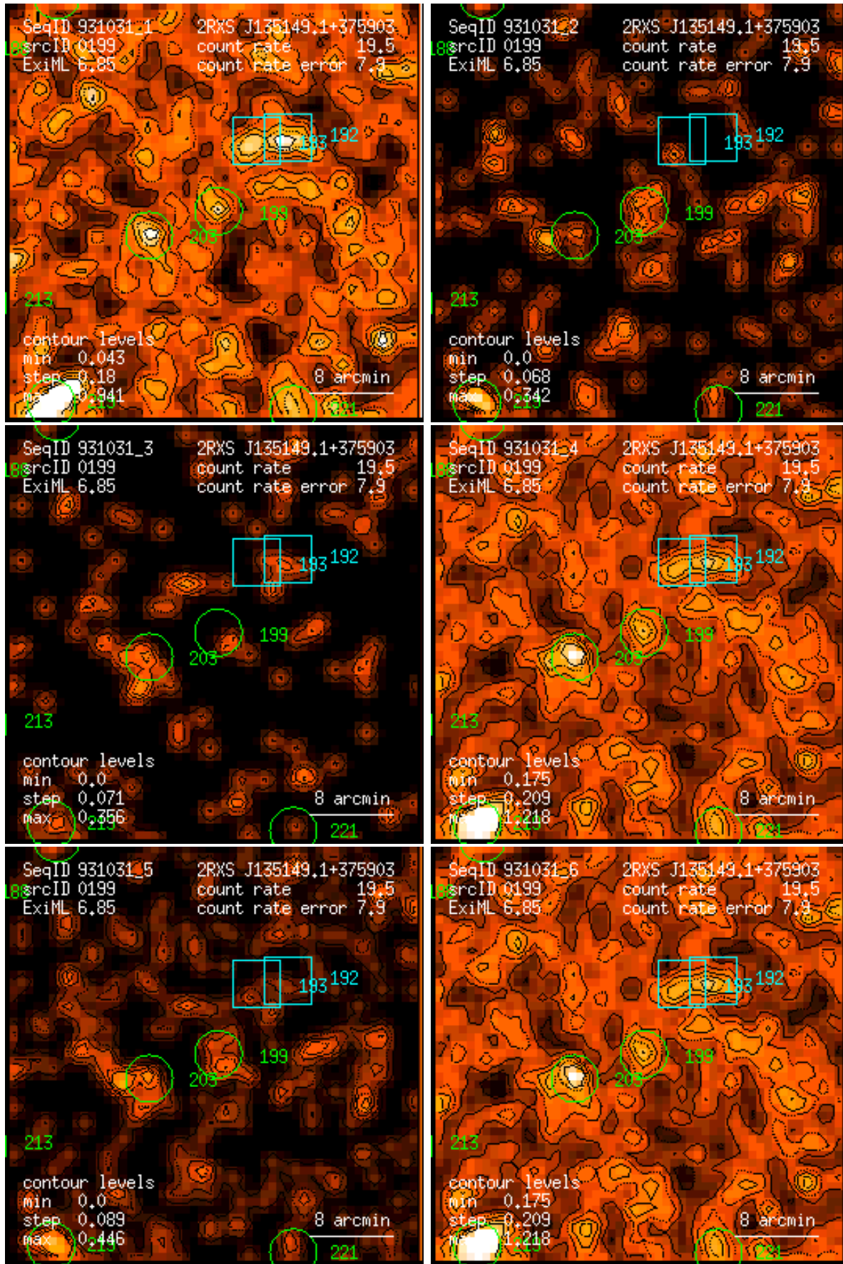
Figure 199: RASS 931031: detection 0199: band rate images, Gaussian filter: (1) PSPC channels 11 – 41, (2) 52 – 90, (3) 91 – 201, (4) 11 – 235, (5) 52 – 201, (6) 11 – 201. Broad band rates in counts/ks. Band rate contour levels in counts/ks/arcmin 2 .
