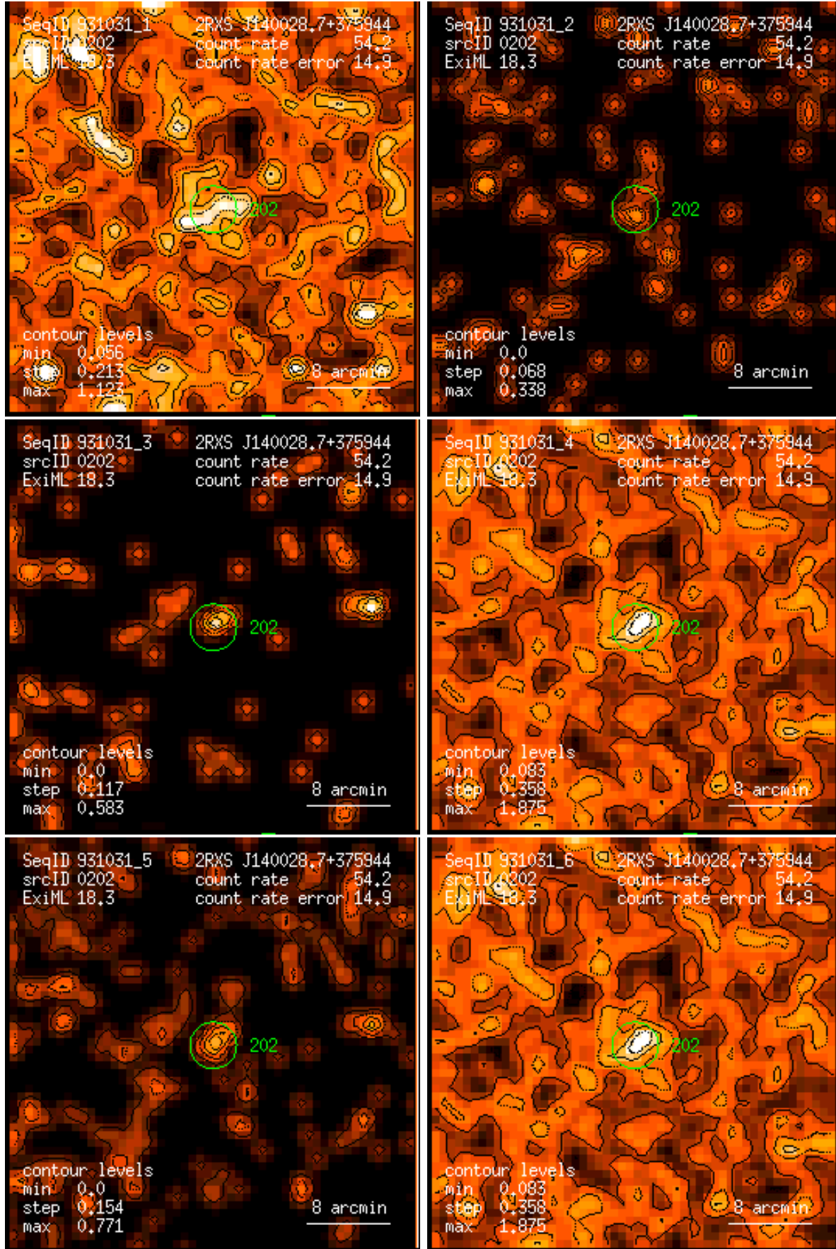
Figure 202: RASS 931031: detection 0202: band rate images, Gaussian filter: (1) PSPC channels 11 – 41, (2) 52 – 90, (3) 91 – 201, (4) 11 – 235, (5) 52 – 201, (6) 11 – 201. Broad band rates in counts/ks. Band rate contour levels in counts/ks/arcmin 2 .
