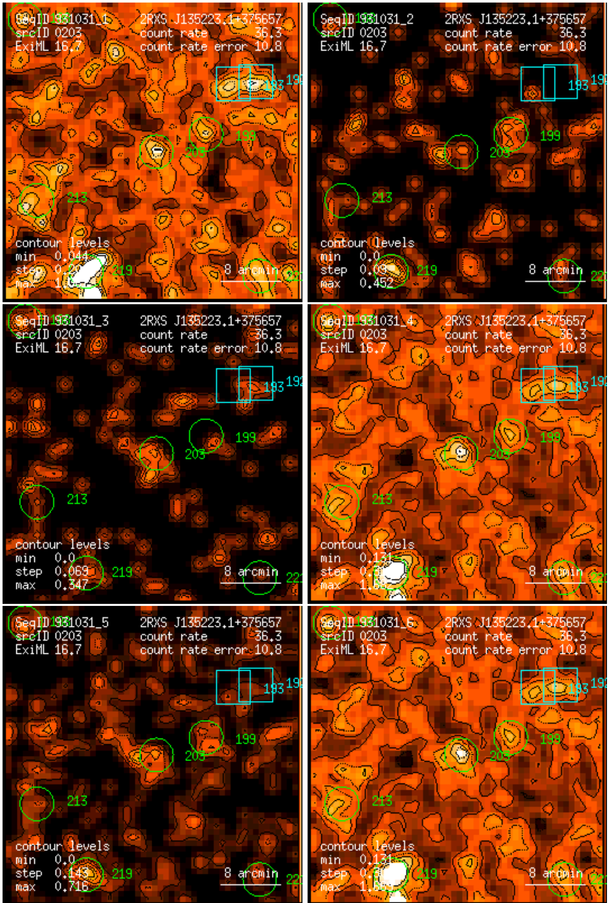
Figure 203: RASS 931031: detection 0203: band rate images, Gaussian filter: (1) PSPC channels 11 – 41, (2) 52 – 90, (3) 91 – 201, (4) 11 – 235, (5) 52 – 201, (6) 11 – 201. Broad band rates in counts/ks. Band rate contour levels in counts/ks/arcmin 2 .
