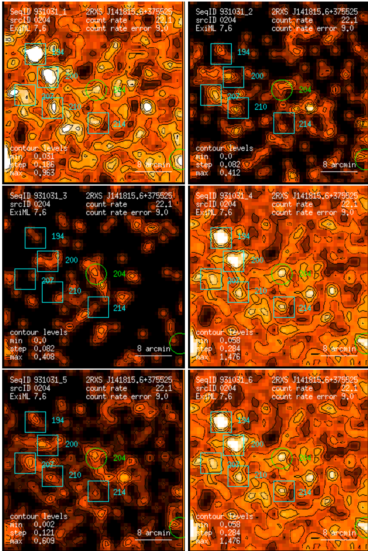
Figure 204: RASS 931031: detection 0204: band rate images, Gaussian filter: (1) PSPC channels 11 – 41, (2) 52 – 90, (3) 91 – 201, (4) 11 – 235, (5) 52 – 201, (6) 11 – 201. Broad band rates in counts/ks. Band rate contour levels in counts/ks/arcmin 2 .
