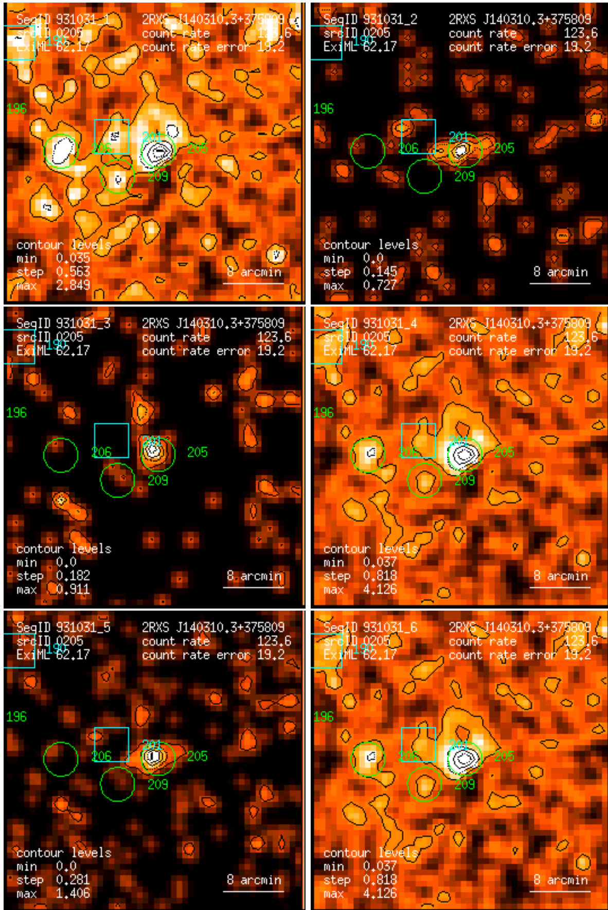
Figure 205: RASS 931031: detection 0205: band rate images, Gaussian filter: (1) PSPC channels 11 – 41, (2) 52 – 90, (3) 91 – 201, (4) 11 – 235, (5) 52 – 201, (6) 11 – 201. Broad band rates in counts/ks. Band rate contour levels in counts/ks/arcmin 2 .
