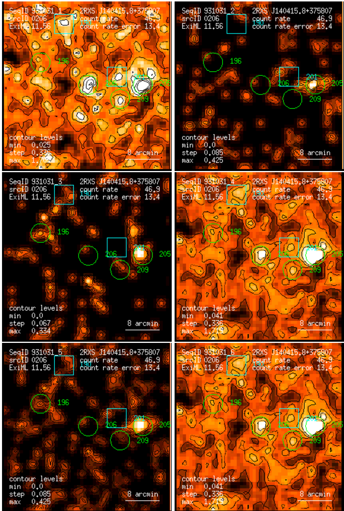
Figure 206: RASS 931031: detection 0206: band rate images, Gaussian filter: (1) PSPC channels 11 – 41, (2) 52 – 90, (3) 91 – 201, (4) 11 – 235, (5) 52 – 201, (6) 11 – 201. Broad band rates in counts/ks. Band rate contour levels in counts/ks/arcmin 2 .
