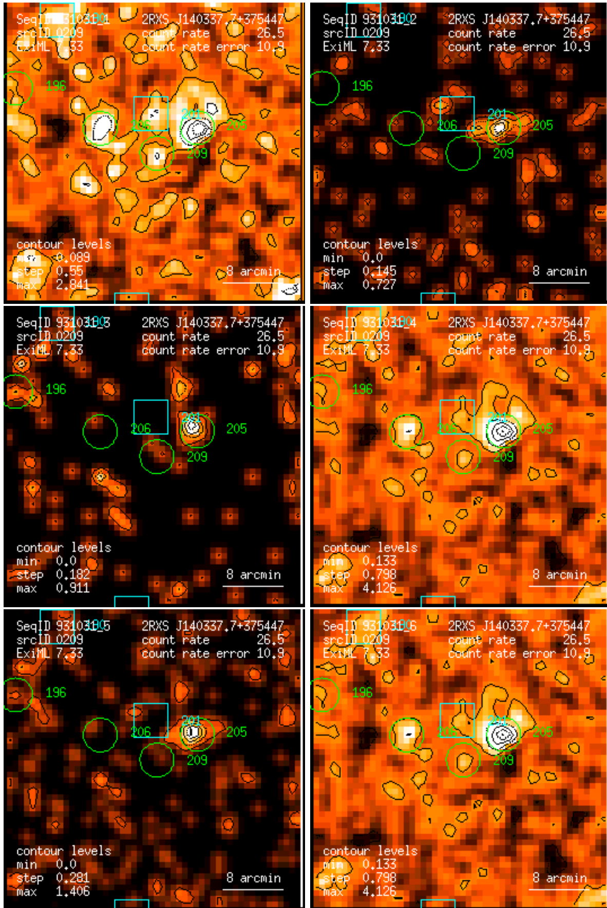
Figure 209: RASS 931031: detection 0209: band rate images, Gaussian filter: (1) PSPC channels 11 – 41, (2) 52 – 90, (3) 91 – 201, (4) 11 – 235, (5) 52 – 201, (6) 11 – 201. Broad band rates in counts/ks. Band rate contour levels in counts/ks/arcmin 2 .
