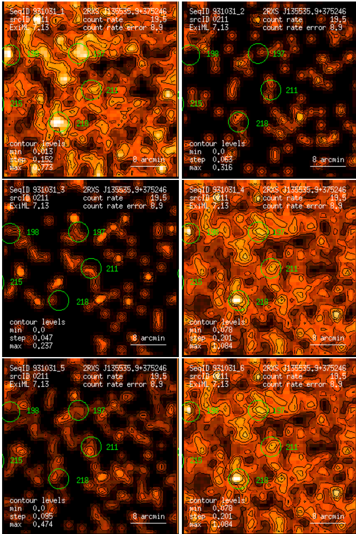
Figure 211: RASS 931031: detection 0211: band rate images, Gaussian filter: (1) PSPC channels 11 – 41, (2) 52 – 90, (3) 91 – 201, (4) 11 – 235, (5) 52 – 201, (6) 11 – 201. Broad band rates in counts/ks. Band rate contour levels in counts/ks/arcmin 2 .
