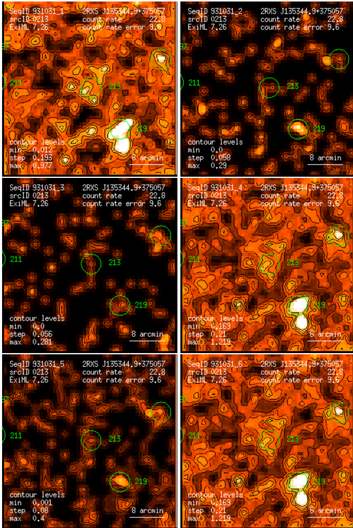
Figure 213: RASS 931031: detection 0213: band rate images, Gaussian filter: (1) PSPC channels 11 – 41, (2) 52 – 90, (3) 91 – 201, (4) 11 – 235, (5) 52 – 201, (6) 11 – 201. Broad band rates in counts/ks. Band rate contour levels in counts/ks/arcmin 2 .
