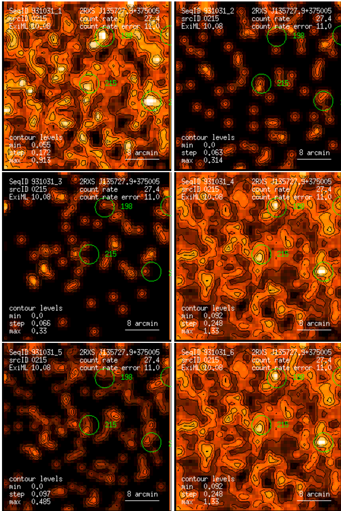
Figure 215: RASS 931031: detection 0215: band rate images, Gaussian filter: (1) PSPC channels 11 – 41, (2) 52 – 90, (3) 91 – 201, (4) 11 – 235, (5) 52 – 201, (6) 11 – 201. Broad band rates in counts/ks. Band rate contour levels in counts/ks/arcmin 2 .
