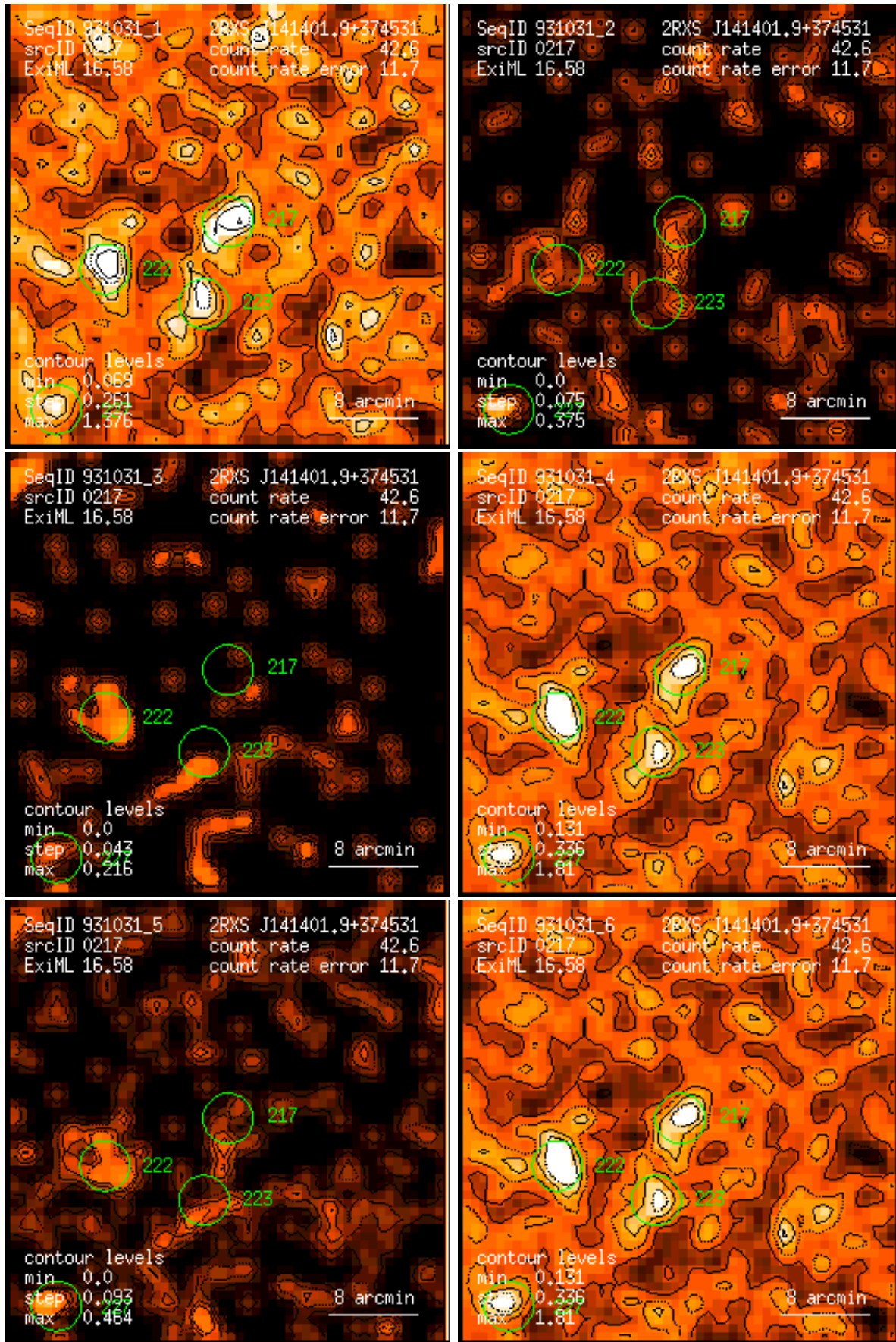
Figure 217: RASS 931031: detection 0217: band rate images, Gaussian filter: (1) PSPC channels 11 – 41, (2) 52 – 90, (3) 91 – 201, (4) 11 – 235, (5) 52 – 201, (6) 11 – 201. Broad band rates in counts/ks. Band rate contour levels in counts/ks/arcmin 2 .
