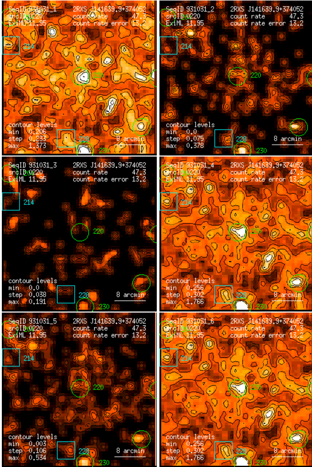
Figure 220: RASS 931031: detection 0220: band rate images, Gaussian filter: (1) PSPC channels 11 – 41, (2) 52 – 90, (3) 91 – 201, (4) 11 – 235, (5) 52 – 201, (6) 11 – 201. Broad band rates in counts/ks. Band rate contour levels in counts/ks/arcmin 2 .
