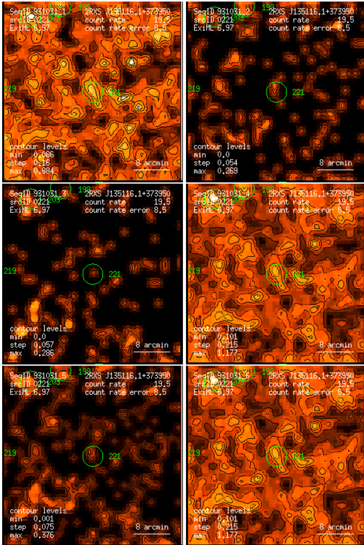
Figure 221: RASS 931031: detection 0221: band rate images, Gaussian filter: (1) PSPC channels 11 – 41, (2) 52 – 90, (3) 91 – 201, (4) 11 – 235, (5) 52 – 201, (6) 11 – 201. Broad band rates in counts/ks. Band rate contour levels in counts/ks/arcmin 2 .
