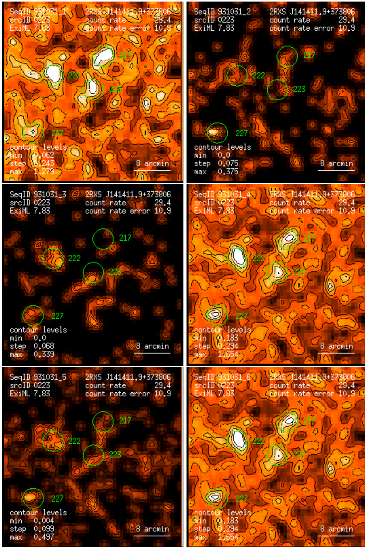
Figure 223: RASS 931031: detection 0223: band rate images, Gaussian filter: (1) PSPC channels 11 – 41, (2) 52 – 90, (3) 91 – 201, (4) 11 – 235, (5) 52 – 201, (6) 11 – 201. Broad band rates in counts/ks. Band rate contour levels in counts/ks/arcmin 2 .
