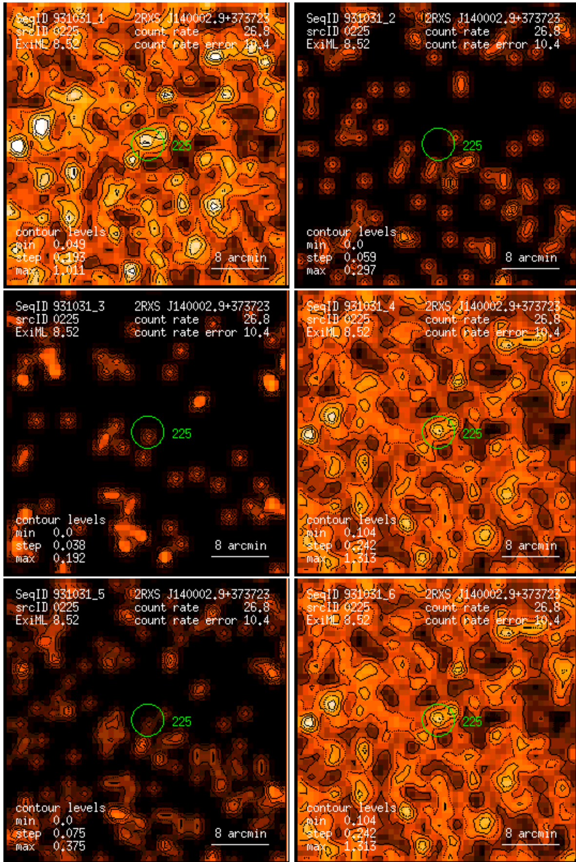
Figure 225: RASS 931031: detection 0225: band rate images, Gaussian filter: (1) PSPC channels 11 – 41, (2) 52 – 90, (3) 91 – 201, (4) 11 – 235, (5) 52 – 201, (6) 11 – 201. Broad band rates in counts/ks. Band rate contour levels in counts/ks/arcmin 2 .
