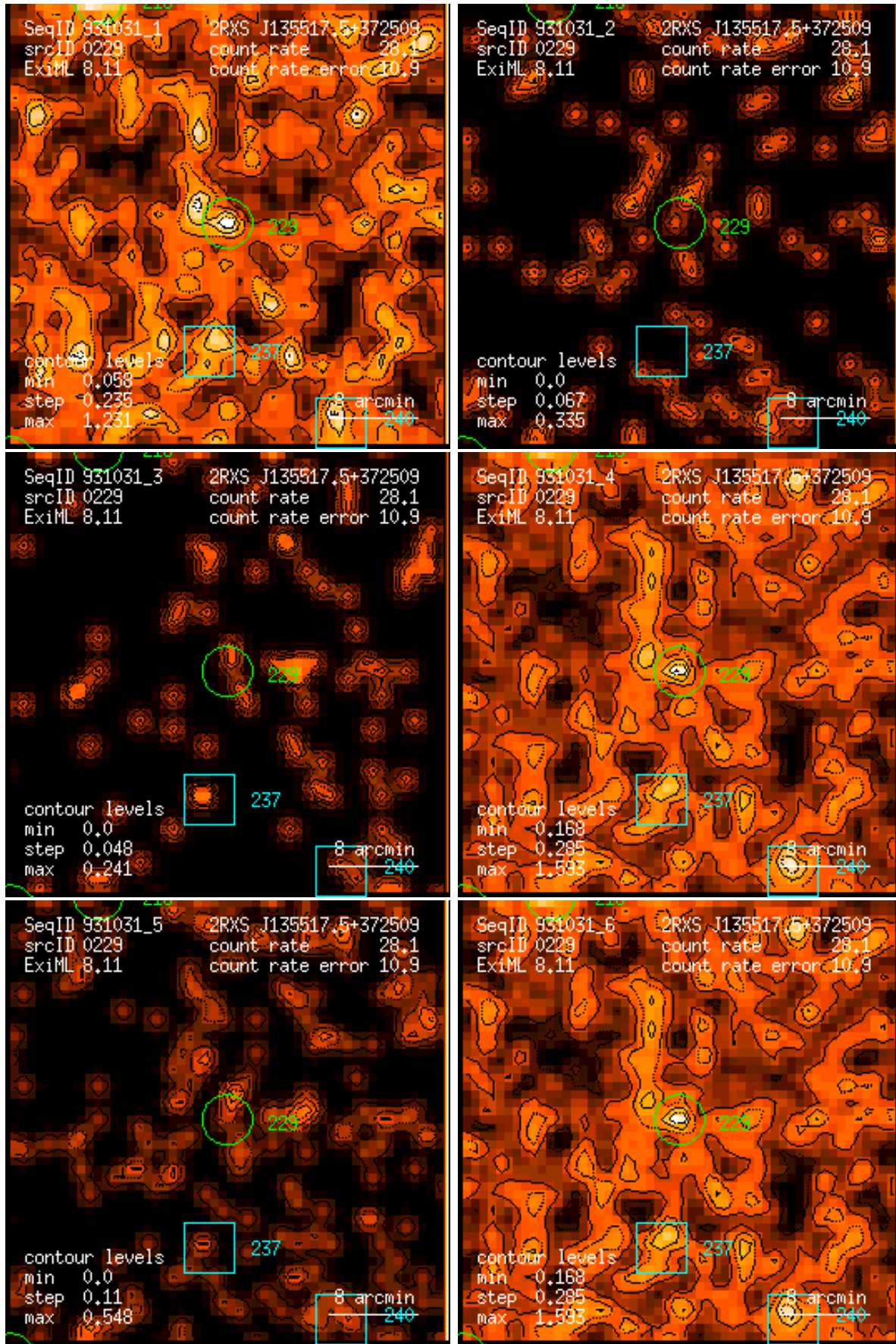
Figure 229: RASS 931031: detection 0229: band rate images, Gaussian filter: (1) PSPC channels 11 – 41, (2) 52 – 90, (3) 91 – 201, (4) 11 – 235, (5) 52 – 201, (6) 11 – 201. Broad band rates in counts/ks. Band rate contour levels in counts/ks/arcmin 2 .
