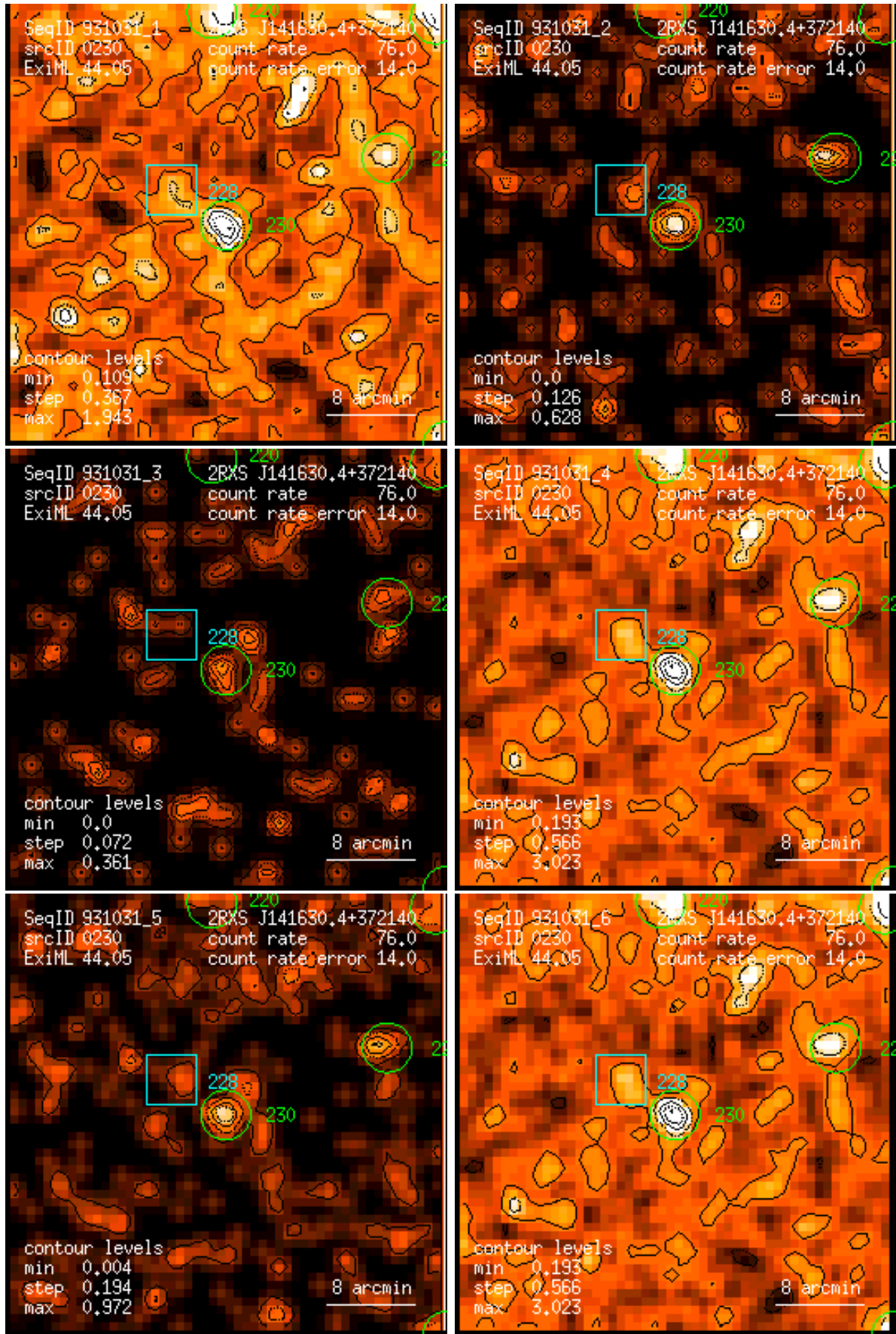
Figure 230: RASS 931031: detection 0230: band rate images, Gaussian filter: (1) PSPC channels 11 – 41, (2) 52 – 90, (3) 91 – 201, (4) 11 – 235, (5) 52 – 201, (6) 11 – 201. Broad band rates in counts/ks. Band rate contour levels in counts/ks/arcmin 2 .
