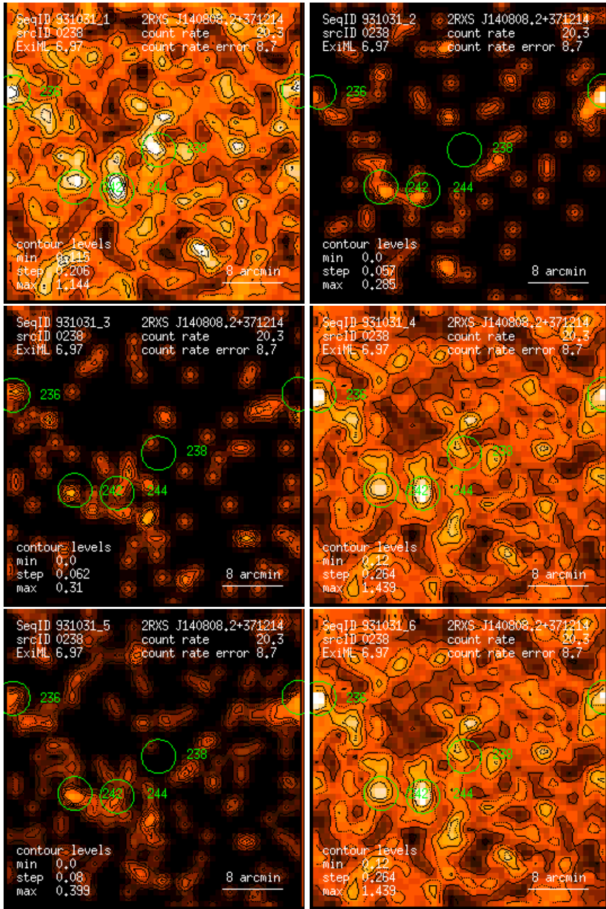
Figure 238: RASS 931031: detection 0238: band rate images, Gaussian filter: (1) PSPC channels 11 – 41, (2) 52 – 90, (3) 91 – 201, (4) 11 – 235, (5) 52 – 201, (6) 11 – 201. Broad band rates in counts/ks. Band rate contour levels in counts/ks/arcmin 2 .
