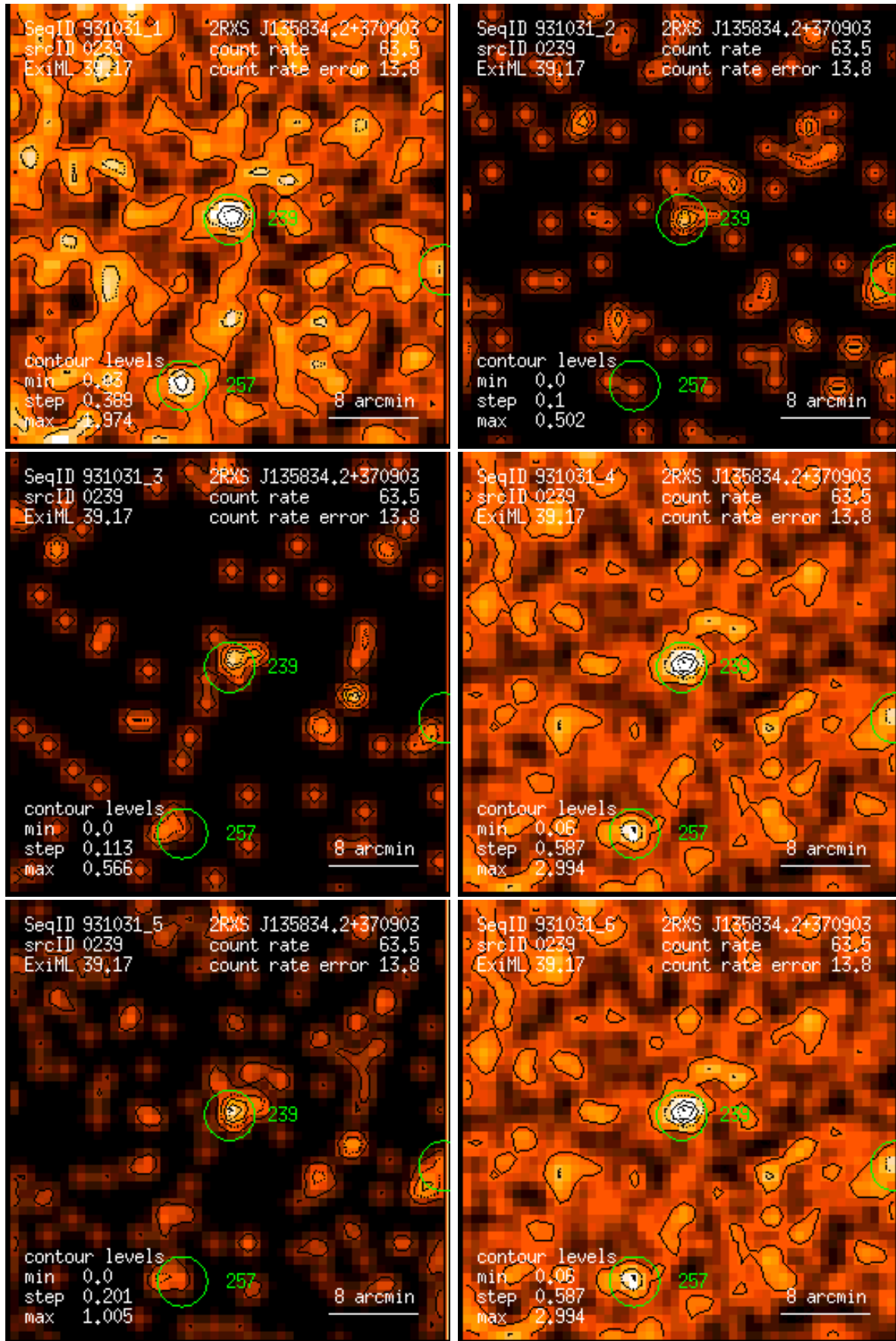
Figure 239: RASS 931031: detection 0239: band rate images, Gaussian filter: (1) PSPC channels 11 – 41, (2) 52 – 90, (3) 91 – 201, (4) 11 – 235, (5) 52 – 201, (6) 11 – 201. Broad band rates in counts/ks. Band rate contour levels in counts/ks/arcmin 2 .
