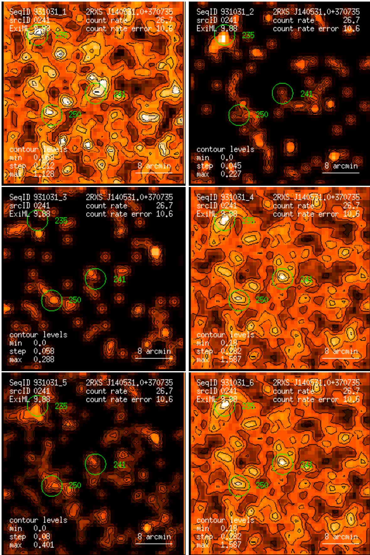
Figure 241: RASS 931031: detection 0241: band rate images, Gaussian filter: (1) PSPC channels 11 – 41, (2) 52 – 90, (3) 91 – 201, (4) 11 – 235, (5) 52 – 201, (6) 11 – 201. Broad band rates in counts/ks. Band rate contour levels in counts/ks/arcmin 2 .
