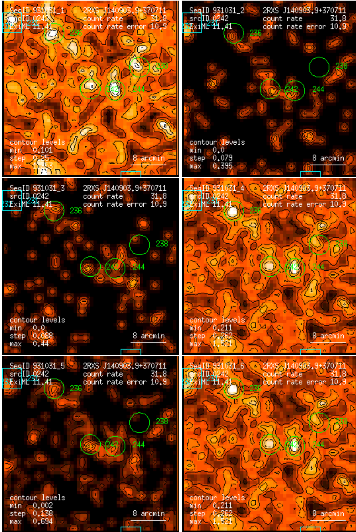
Figure 242: RASS 931031: detection 0242: band rate images, Gaussian filter: (1) PSPC channels 11 – 41, (2) 52 – 90, (3) 91 – 201, (4) 11 – 235, (5) 52 – 201, (6) 11 – 201. Broad band rates in counts/ks. Band rate contour levels in counts/ks/arcmin 2 .
