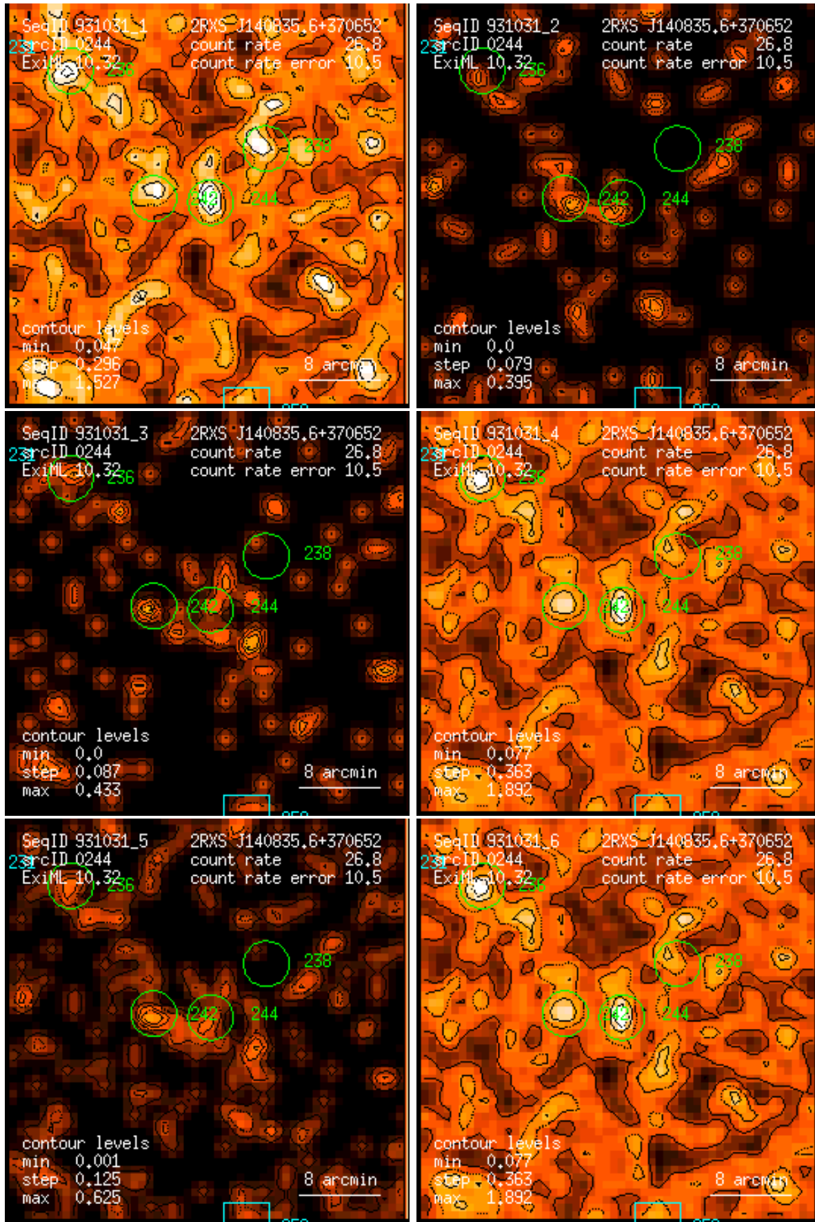
Figure 244: RASS 931031: detection 0244: band rate images, Gaussian filter: (1) PSPC channels 11 – 41, (2) 52 – 90, (3) 91 – 201, (4) 11 – 235, (5) 52 – 201, (6) 11 – 201. Broad band rates in counts/ks. Band rate contour levels in counts/ks/arcmin 2 .
