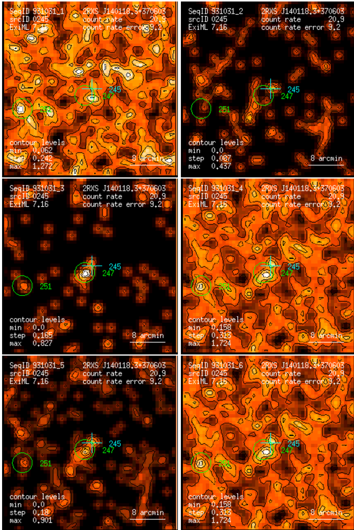
Figure 245: RASS 931031: detection 0245: band rate images, Gaussian filter: (1) PSPC channels 11 – 41, (2) 52 – 90, (3) 91 – 201, (4) 11 – 235, (5) 52 – 201, (6) 11 – 201. Broad band rates in counts/ks. Band rate contour levels in counts/ks/arcmin 2 .
