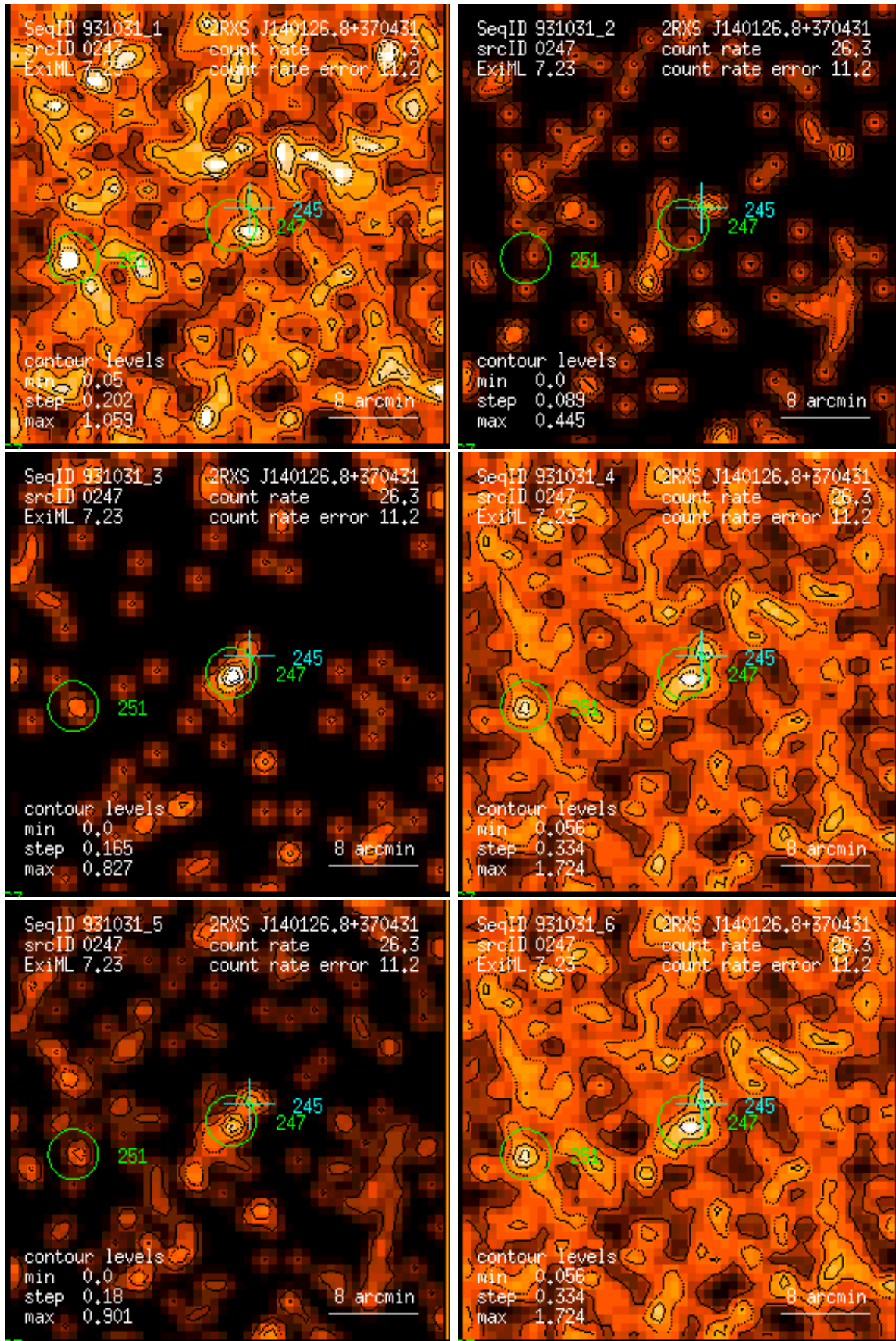
Figure 247: RASS 931031: detection 0247: band rate images, Gaussian filter: (1) PSPC channels 11 – 41, (2) 52 – 90, (3) 91 – 201, (4) 11 – 235, (5) 52 – 201, (6) 11 – 201. Broad band rates in counts/ks. Band rate contour levels in counts/ks/arcmin 2 .
