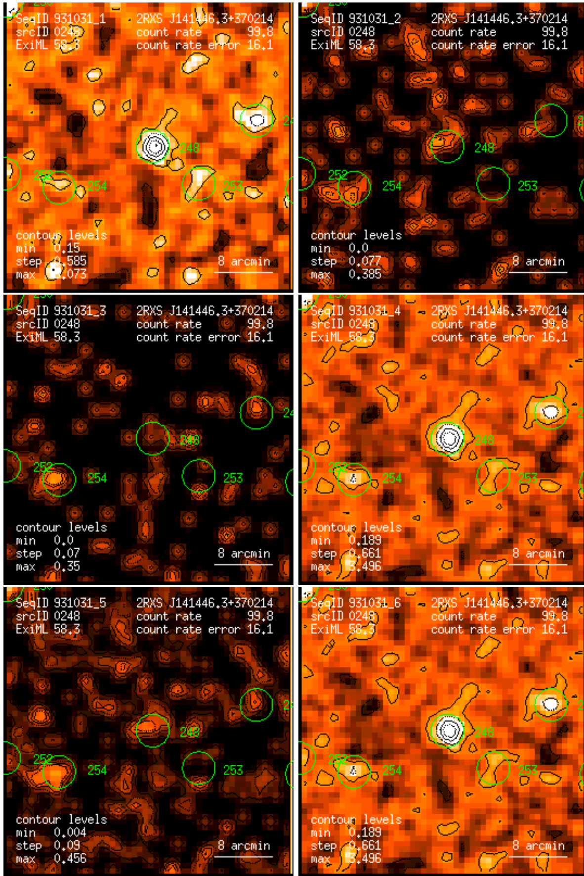
Figure 248: RASS 931031: detection 0248: band rate images, Gaussian filter: (1) PSPC channels 11 – 41, (2) 52 – 90, (3) 91 – 201, (4) 11 – 235, (5) 52 – 201, (6) 11 – 201. Broad band rates in counts/ks. Band rate contour levels in counts/ks/arcmin 2 .
