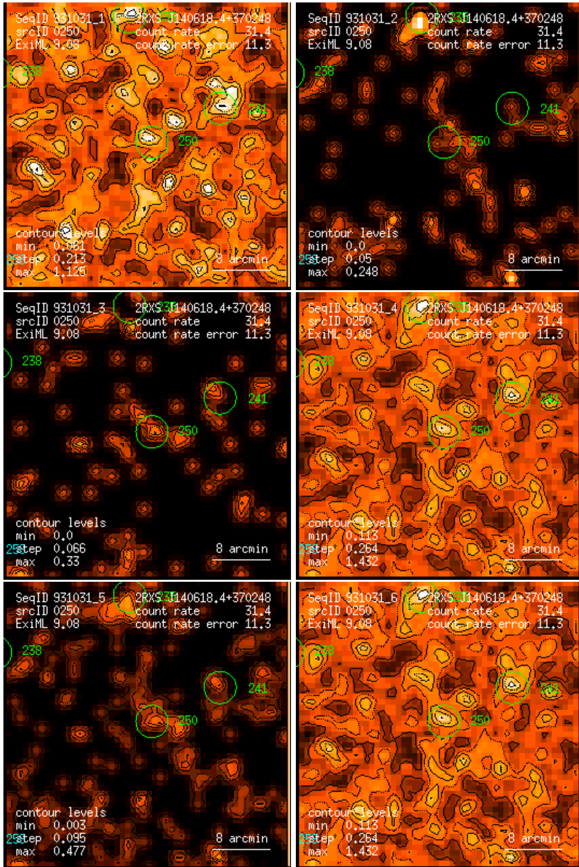
Figure 250: RASS 931031: detection 0250: band rate images, Gaussian filter: (1) PSPC channels 11 – 41, (2) 52 – 90, (3) 91 – 201, (4) 11 – 235, (5) 52 – 201, (6) 11 – 201. Broad band rates in counts/ks. Band rate contour levels in counts/ks/arcmin 2 .
