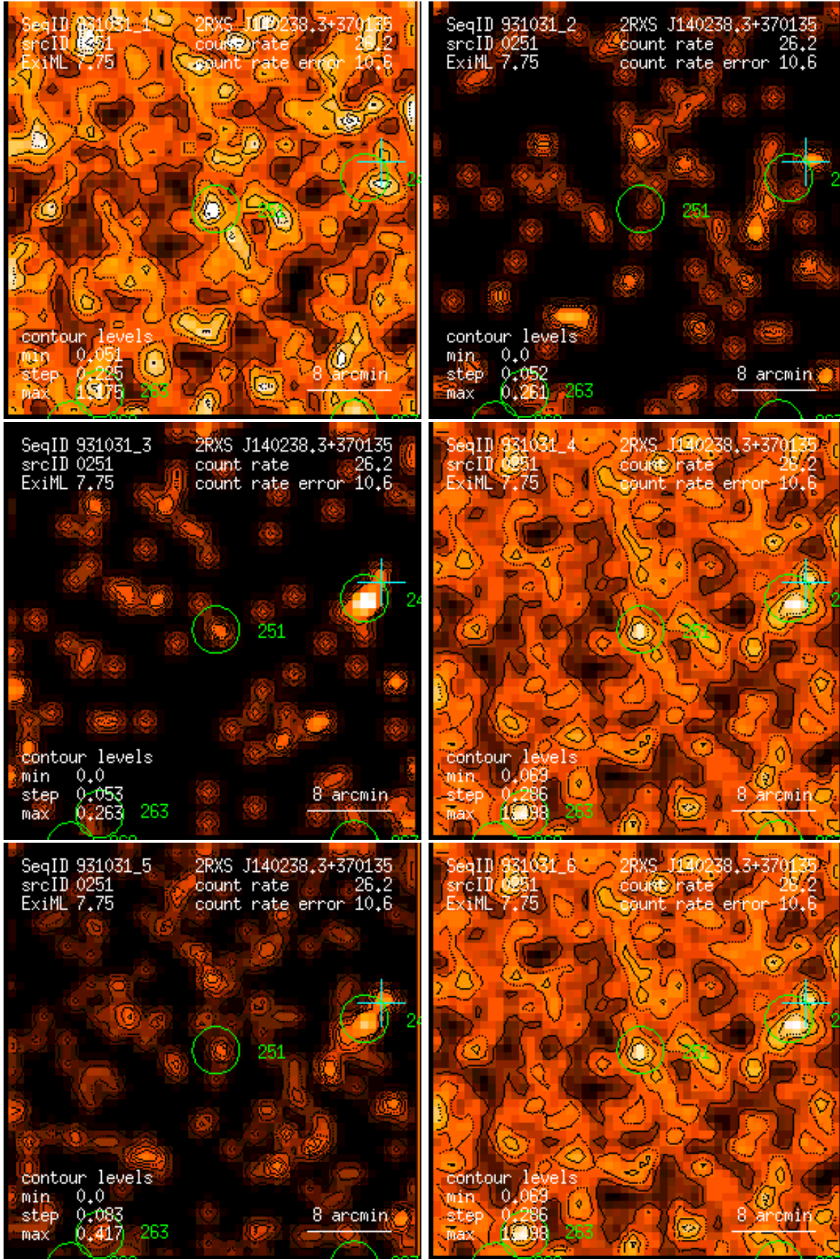
Figure 251: RASS 931031: detection 0251: band rate images, Gaussian filter: (1) PSPC channels 11 – 41, (2) 52 – 90, (3) 91 – 201, (4) 11 – 235, (5) 52 – 201, (6) 11 – 201. Broad band rates in counts/ks. Band rate contour levels in counts/ks/arcmin 2 .
