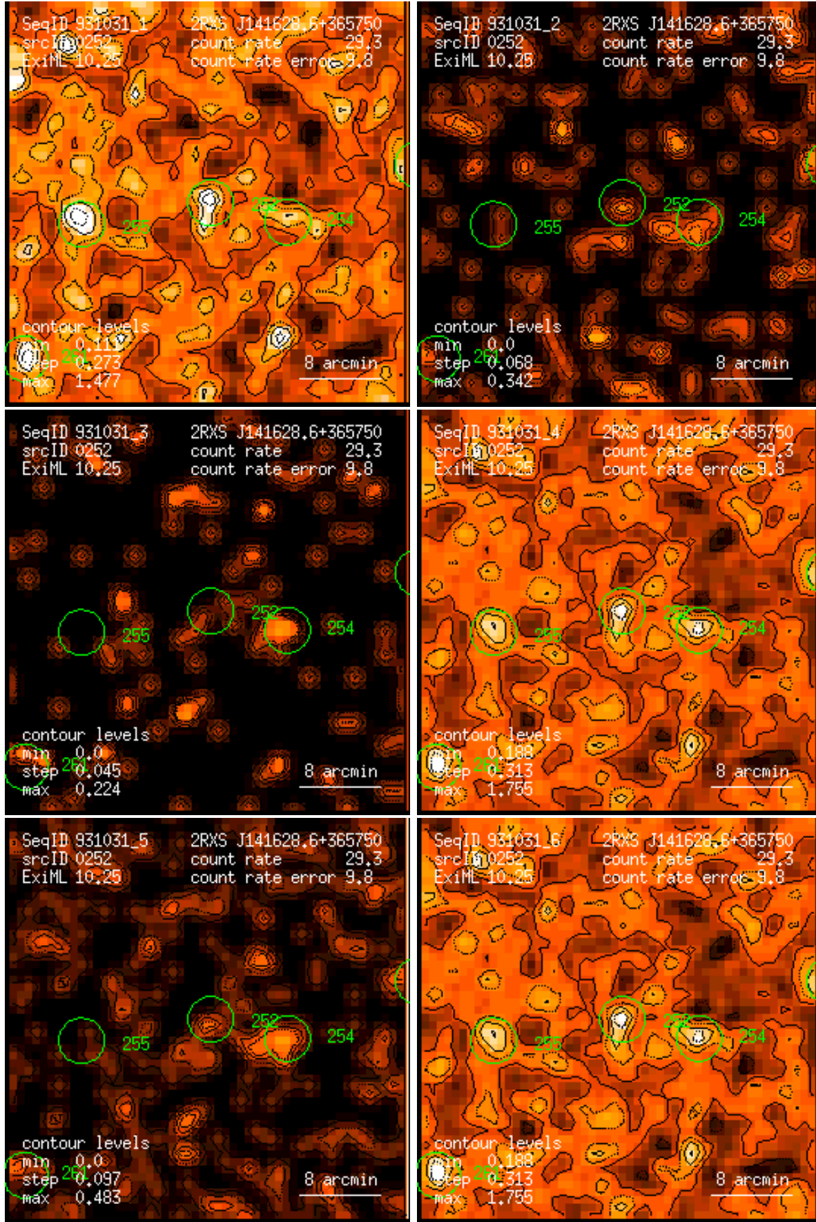
Figure 252: RASS 931031: detection 0252: band rate images, Gaussian filter: (1) PSPC channels 11 – 41, (2) 52 – 90, (3) 91 – 201, (4) 11 – 235, (5) 52 – 201, (6) 11 – 201. Broad band rates in counts/ks. Band rate contour levels in counts/ks/arcmin 2 .
