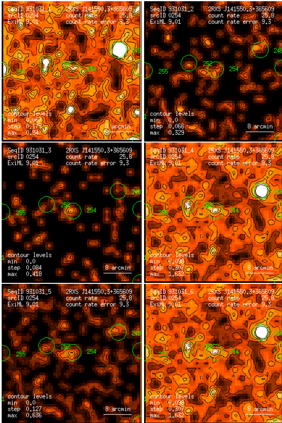
Figure 254: RASS 931031: detection 0254: band rate images, Gaussian filter: (1) PSPC channels 11 – 41, (2) 52 – 90, (3) 91 – 201, (4) 11 – 235, (5) 52 – 201, (6) 11 – 201. Broad band rates in counts/ks. Band rate contour levels in counts/ks/arcmin 2 .
