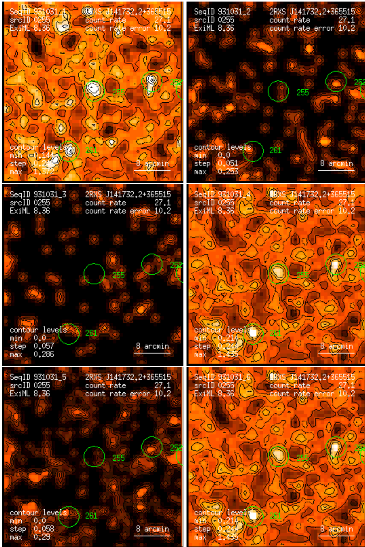
Figure 255: RASS 931031: detection 0255: band rate images, Gaussian filter: (1) PSPC channels 11 – 41, (2) 52 – 90, (3) 91 – 201, (4) 11 – 235, (5) 52 – 201, (6) 11 – 201. Broad band rates in counts/ks. Band rate contour levels in counts/ks/arcmin 2 .
