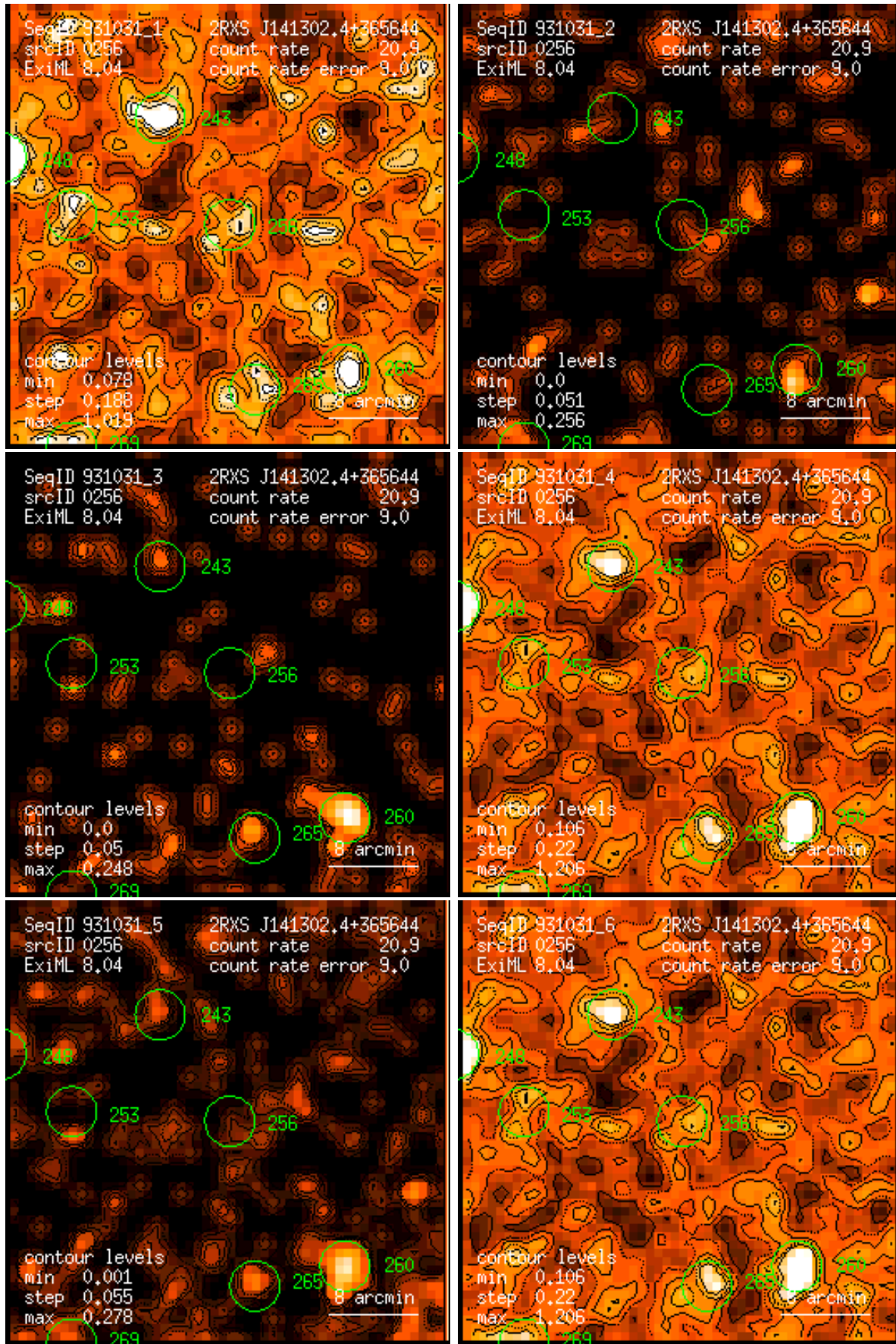
Figure 256: RASS 931031: detection 0256: band rate images, Gaussian filter: (1) PSPC channels 11 – 41, (2) 52 – 90, (3) 91 – 201, (4) 11 – 235, (5) 52 – 201, (6) 11 – 201. Broad band rates in counts/ks. Band rate contour levels in counts/ks/arcmin 2 .
