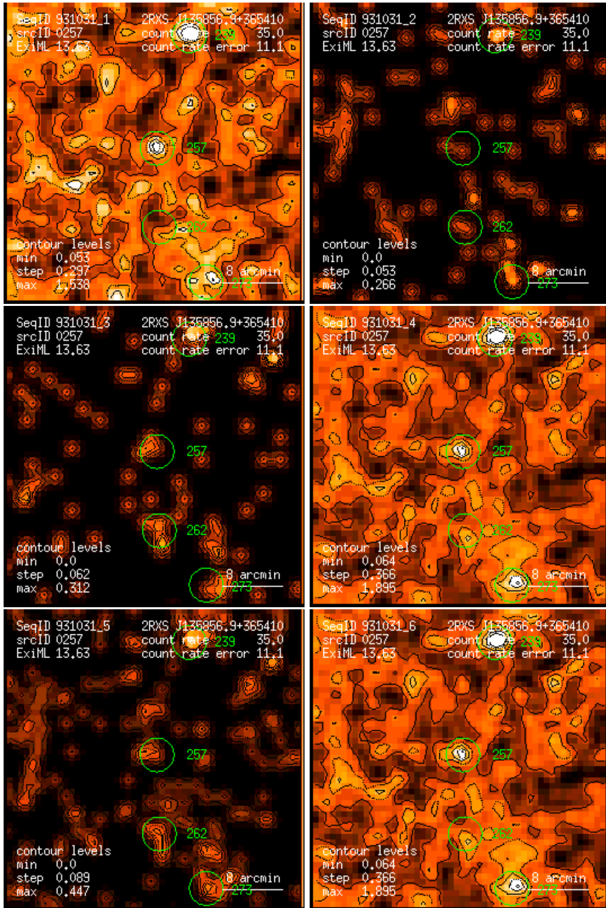
Figure 257: RASS 931031: detection 0257: band rate images, Gaussian filter: (1) PSPC channels 11 – 41, (2) 52 – 90, (3) 91 – 201, (4) 11 – 235, (5) 52 – 201, (6) 11 – 201. Broad band rates in counts/ks. Band rate contour levels in counts/ks/arcmin 2 .
