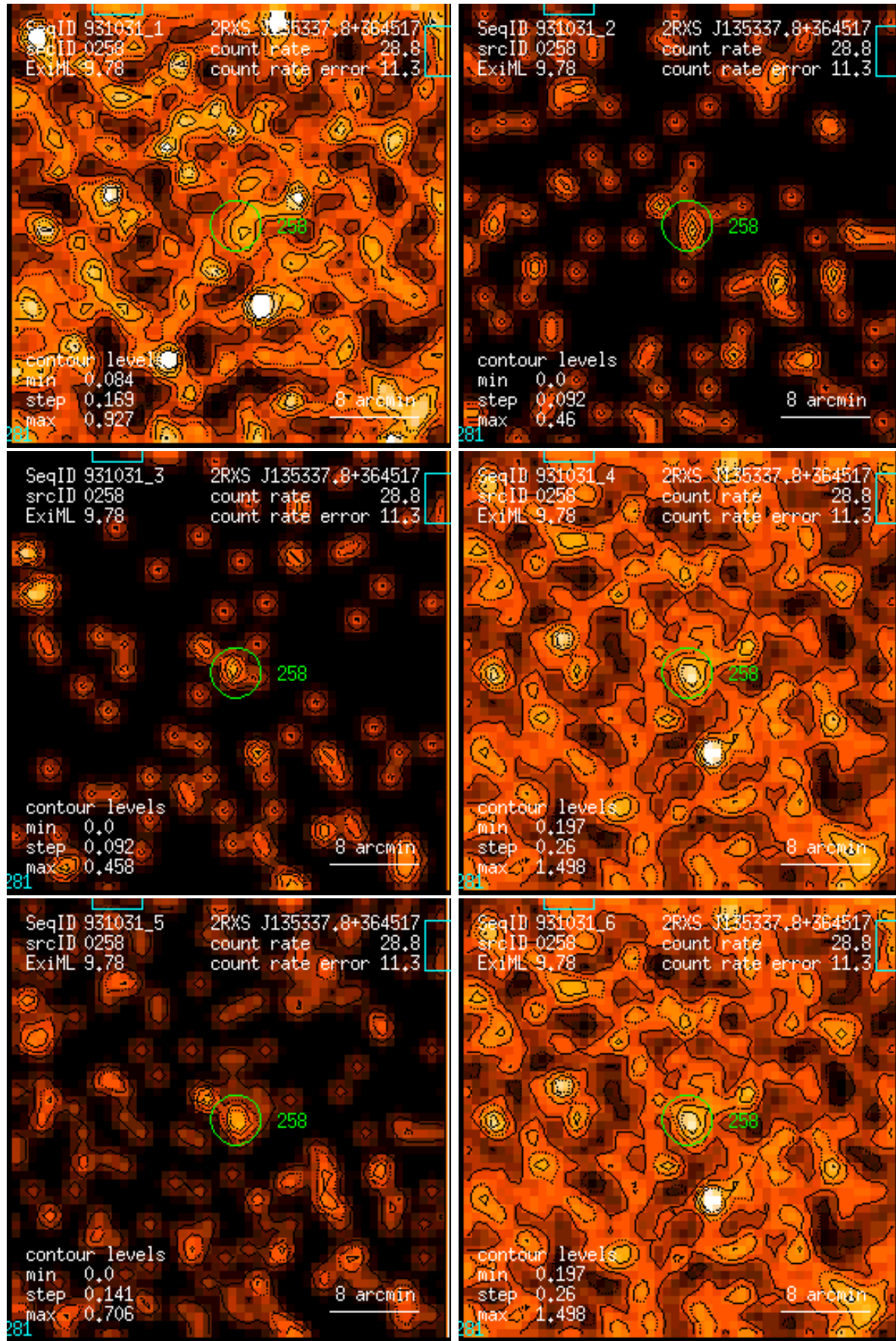
Figure 258: RASS 931031: detection 0258: band rate images, Gaussian filter: (1) PSPC channels 11 – 41, (2) 52 – 90, (3) 91 – 201, (4) 11 – 235, (5) 52 – 201, (6) 11 – 201. Broad band rates in counts/ks. Band rate contour levels in counts/ks/arcmin 2 .
