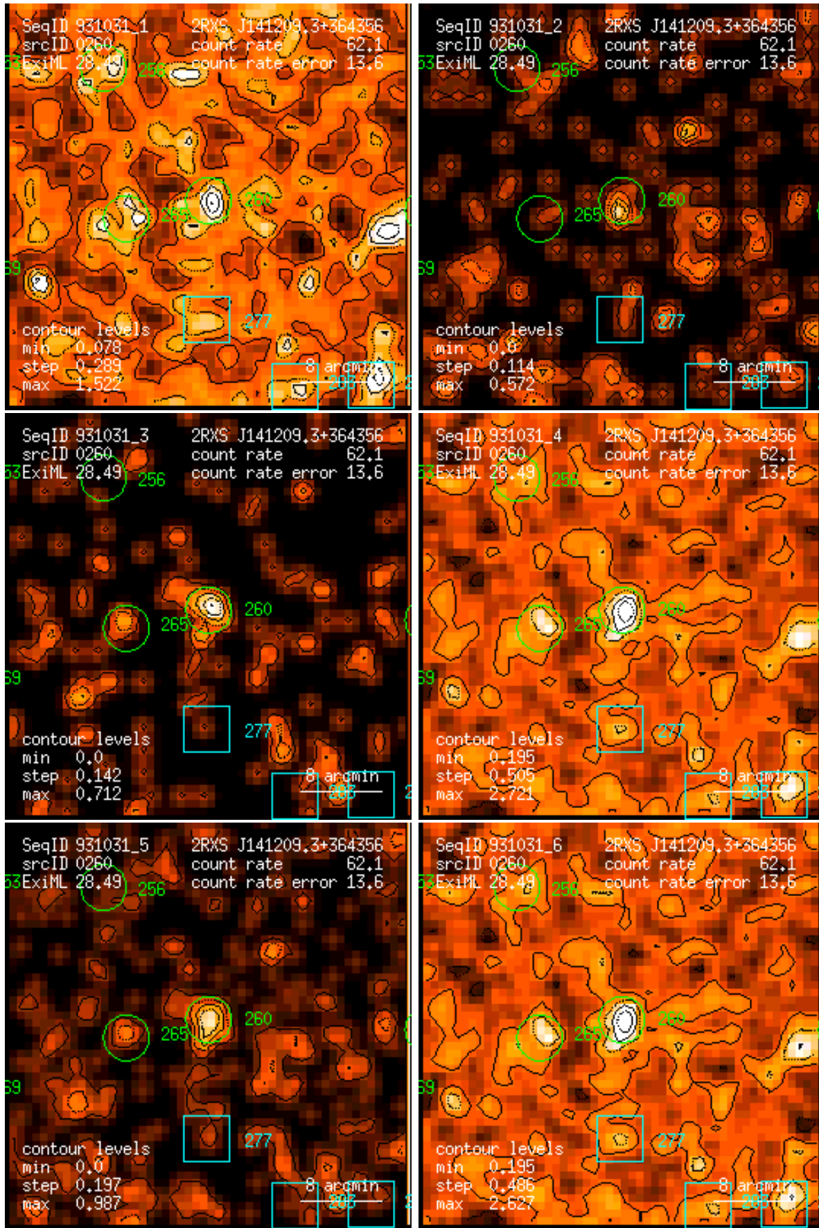
Figure 260: RASS 931031: detection 0260: band rate images, Gaussian filter: (1) PSPC channels 11 – 41, (2) 52 – 90, (3) 91 – 201, (4) 11 – 235, (5) 52 – 201, (6) 11 – 201. Broad band rates in counts/ks. Band rate contour levels in counts/ks/arcmin 2 .
