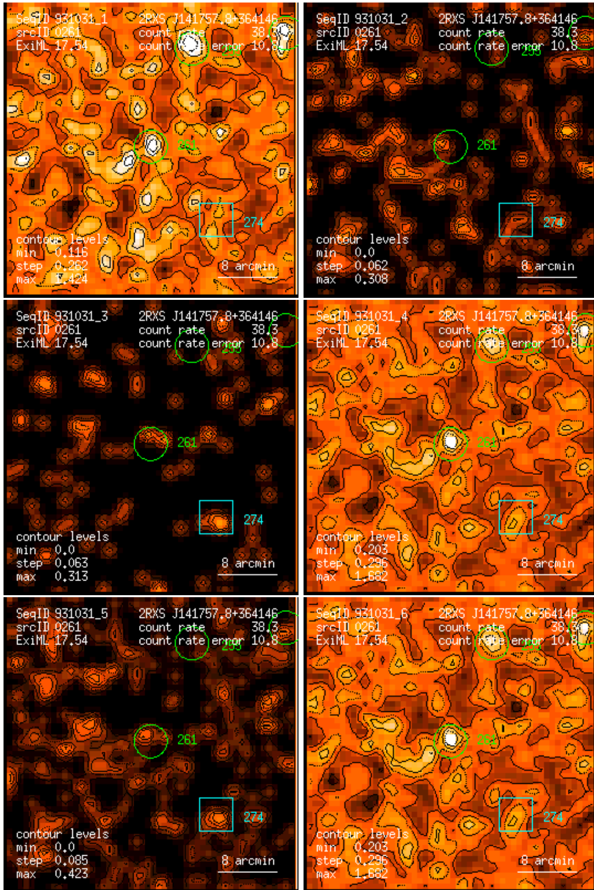
Figure 261: RASS 931031: detection 0261: band rate images, Gaussian filter: (1) PSPC channels 11 – 41, (2) 52 – 90, (3) 91 – 201, (4) 11 – 235, (5) 52 – 201, (6) 11 – 201. Broad band rates in counts/ks. Band rate contour levels in counts/ks/arcmin 2 .
