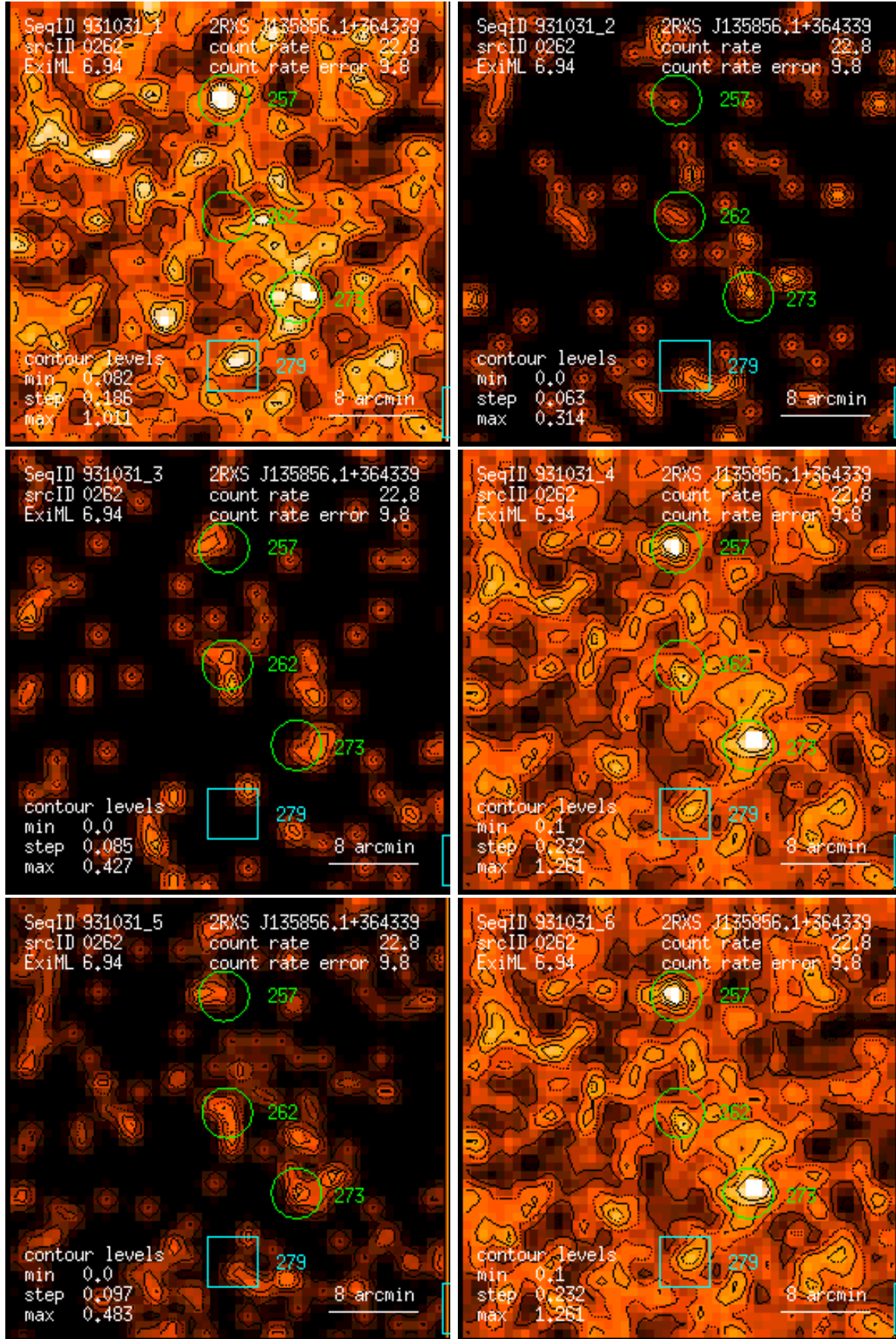
Figure 262: RASS 931031: detection 0262: band rate images, Gaussian filter: (1) PSPC channels 11 – 41, (2) 52 – 90, (3) 91 – 201, (4) 11 – 235, (5) 52 – 201, (6) 11 – 201. Broad band rates in counts/ks. Band rate contour levels in counts/ks/arcmin 2 .
