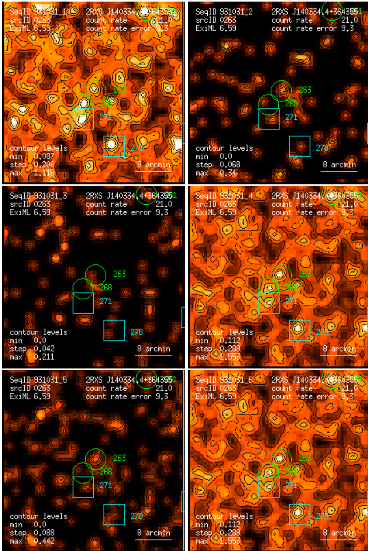
Figure 263: RASS 931031: detection 0263: band rate images, Gaussian filter: (1) PSPC channels 11 – 41, (2) 52 – 90, (3) 91 – 201, (4) 11 – 235, (5) 52 – 201, (6) 11 – 201. Broad band rates in counts/ks. Band rate contour levels in counts/ks/arcmin 2 .
