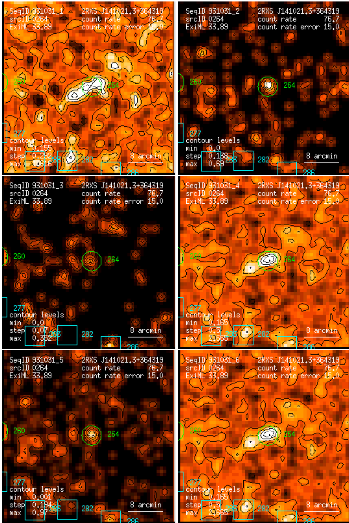
Figure 264: RASS 931031: detection 0264: band rate images, Gaussian filter: (1) PSPC channels 11 – 41, (2) 52 – 90, (3) 91 – 201, (4) 11 – 235, (5) 52 – 201, (6) 11 – 201. Broad band rates in counts/ks. Band rate contour levels in counts/ks/arcmin 2 .
